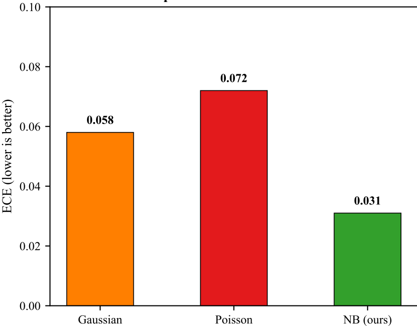
Expected Calibration Error
