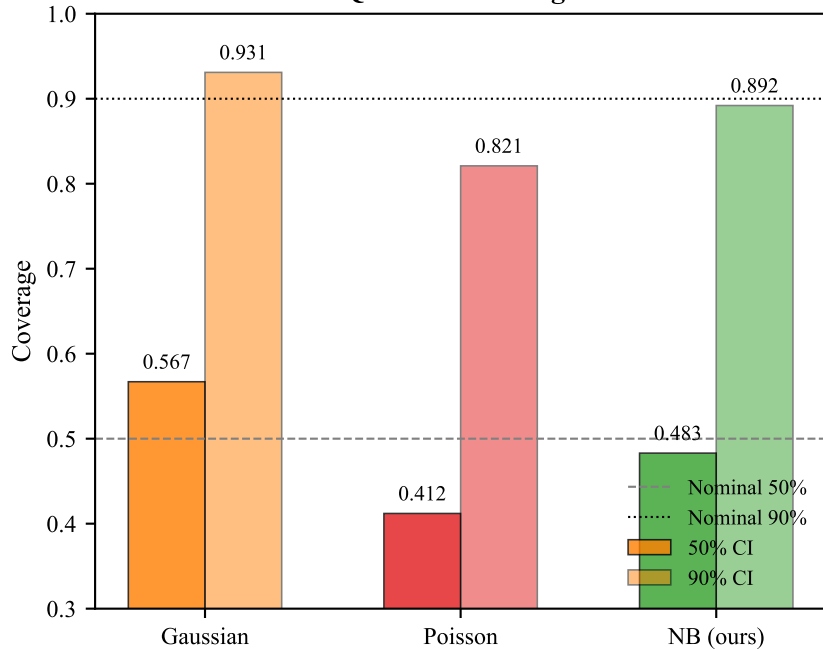
Quantile Coverage
