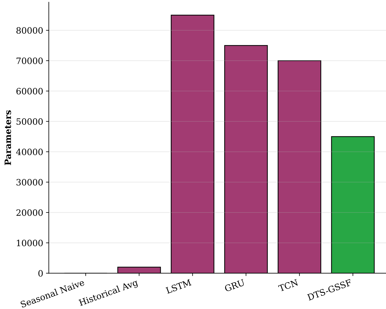
Model Complexity Comparison
