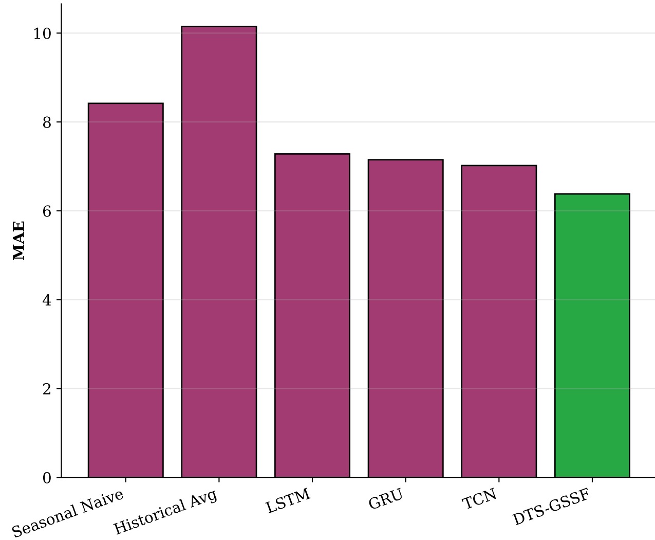
Model Performance Comparison
