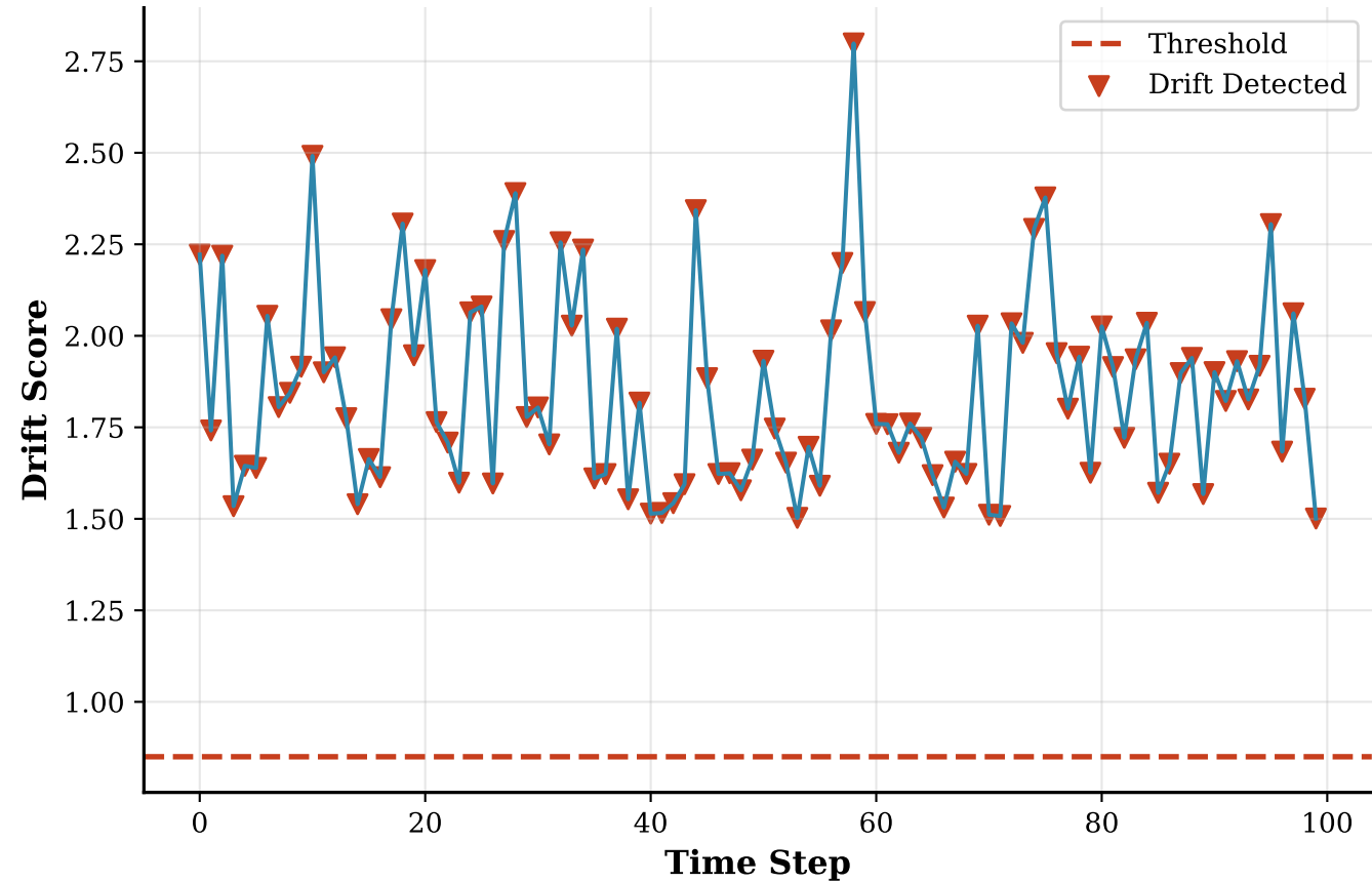
Concept Drift Detection
