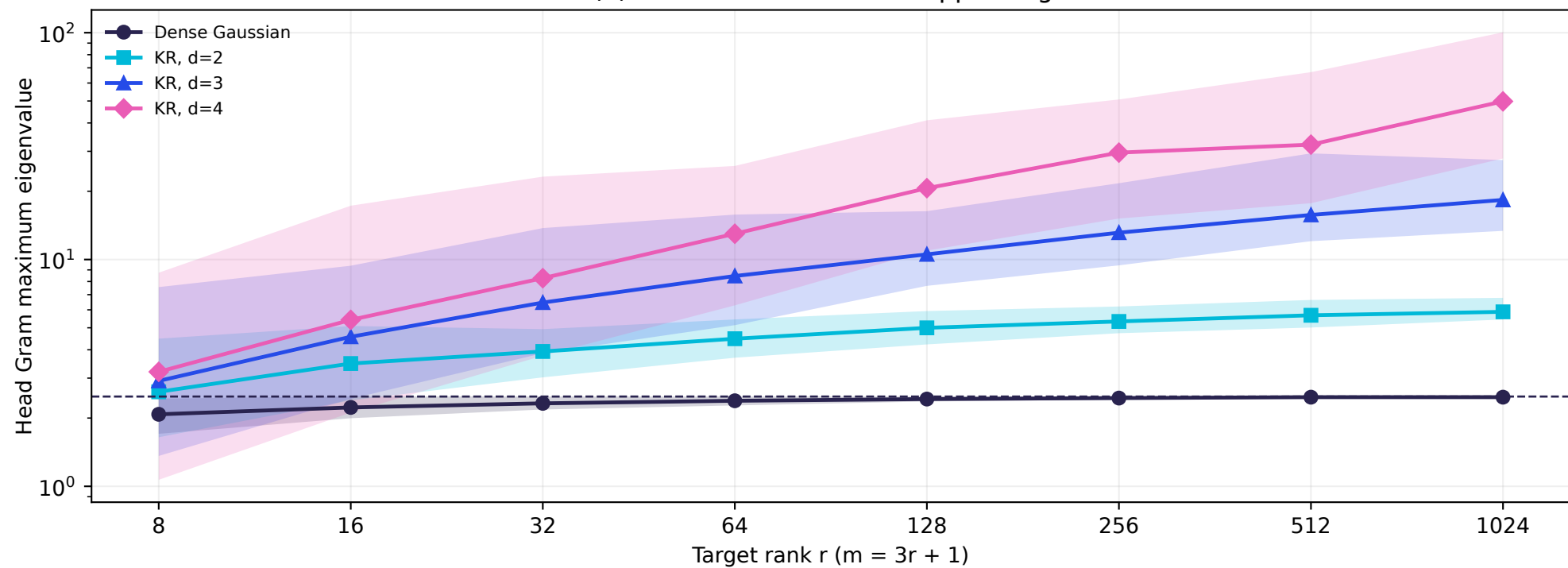
(b) Same input: rank-r approximation
