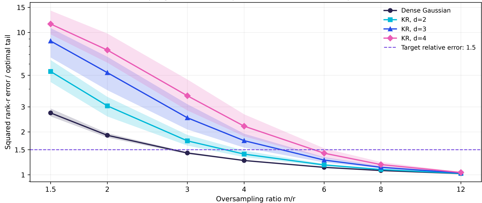
Oversampling on one fixed input ( r = 32 ; common-mode product 512)
