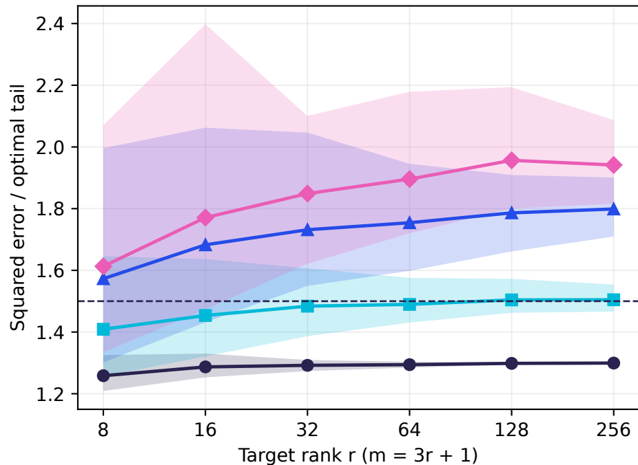
Same input: rank-r approximation
