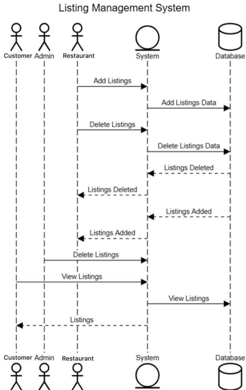
Figure 11 Sequence Diagram LM
