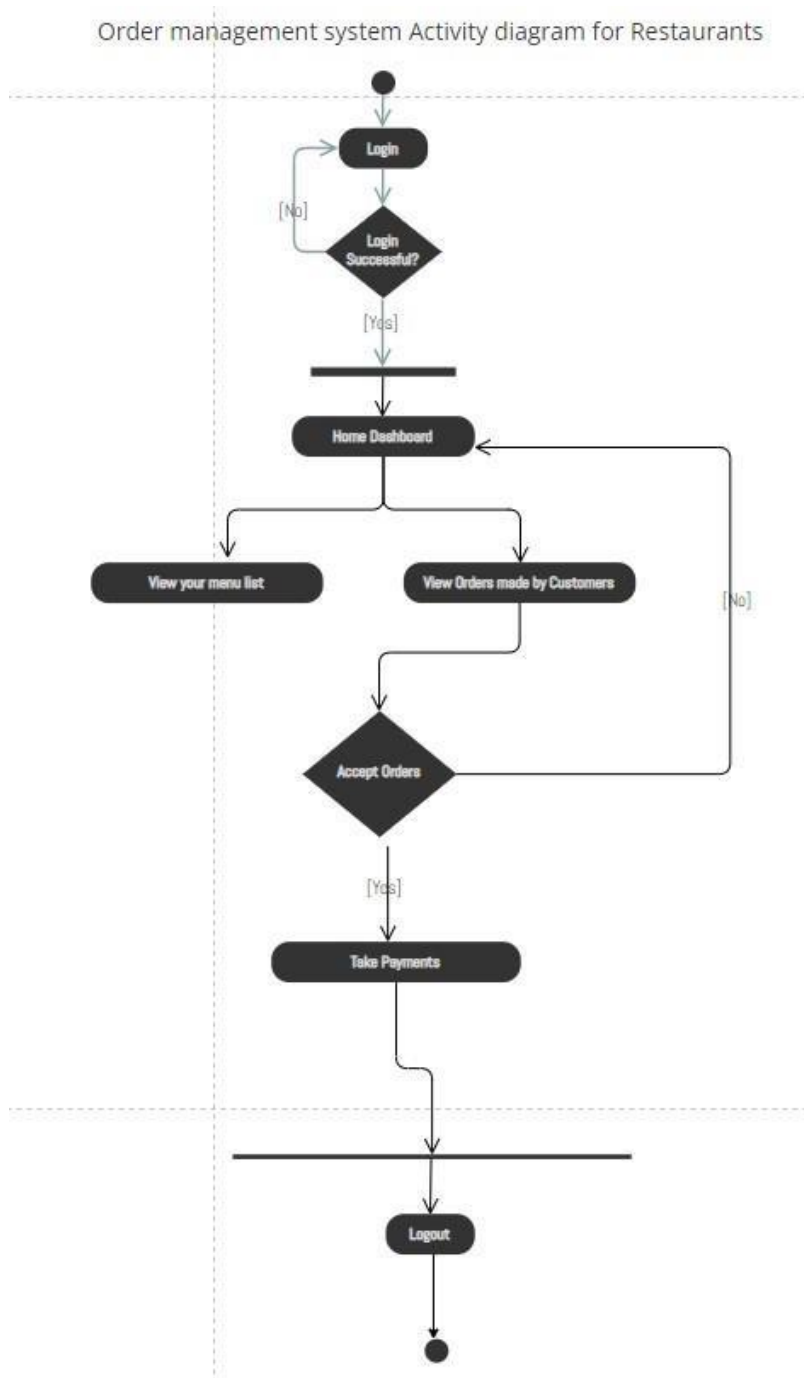
Figure 13 Activity Diagram restaurants OM
