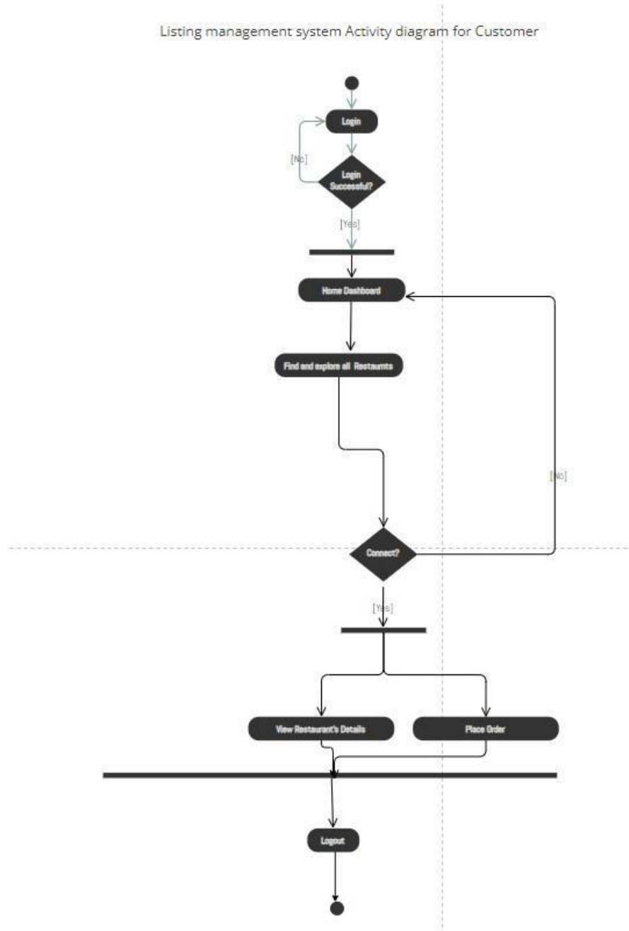
Figure 7 Activity Diagram for Customer LM
