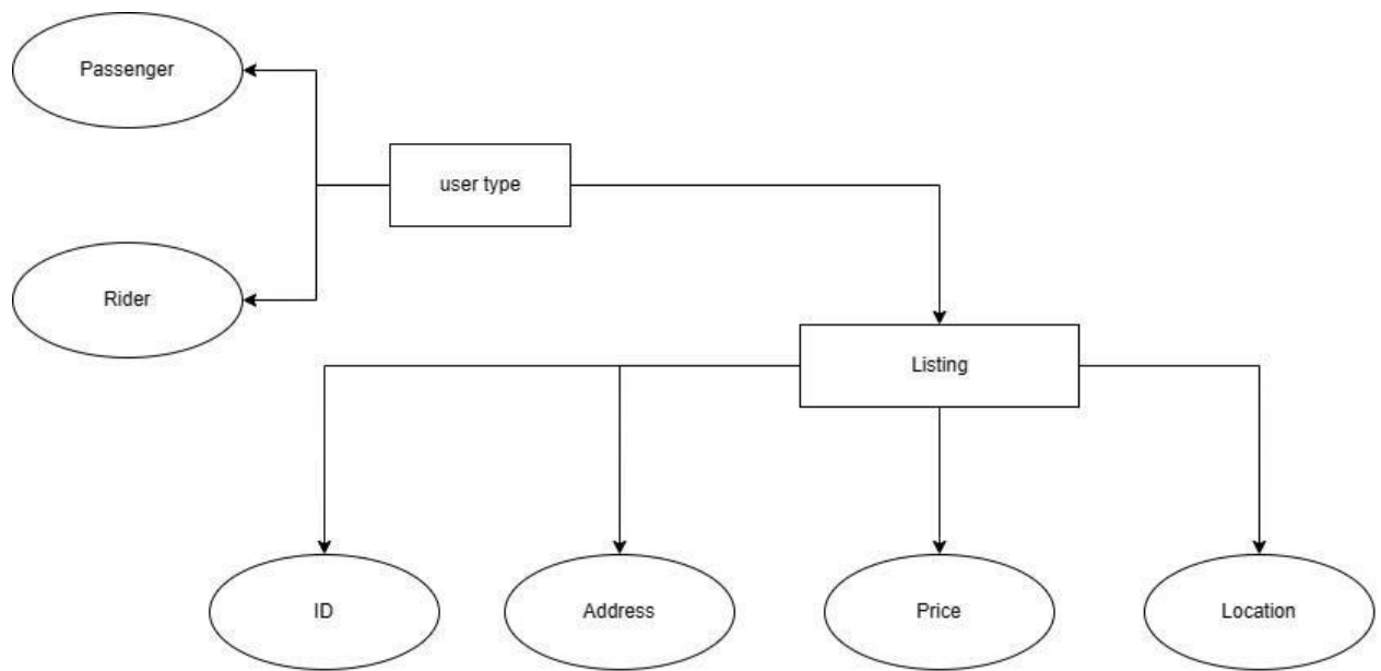
Figure 10 ERD LM
