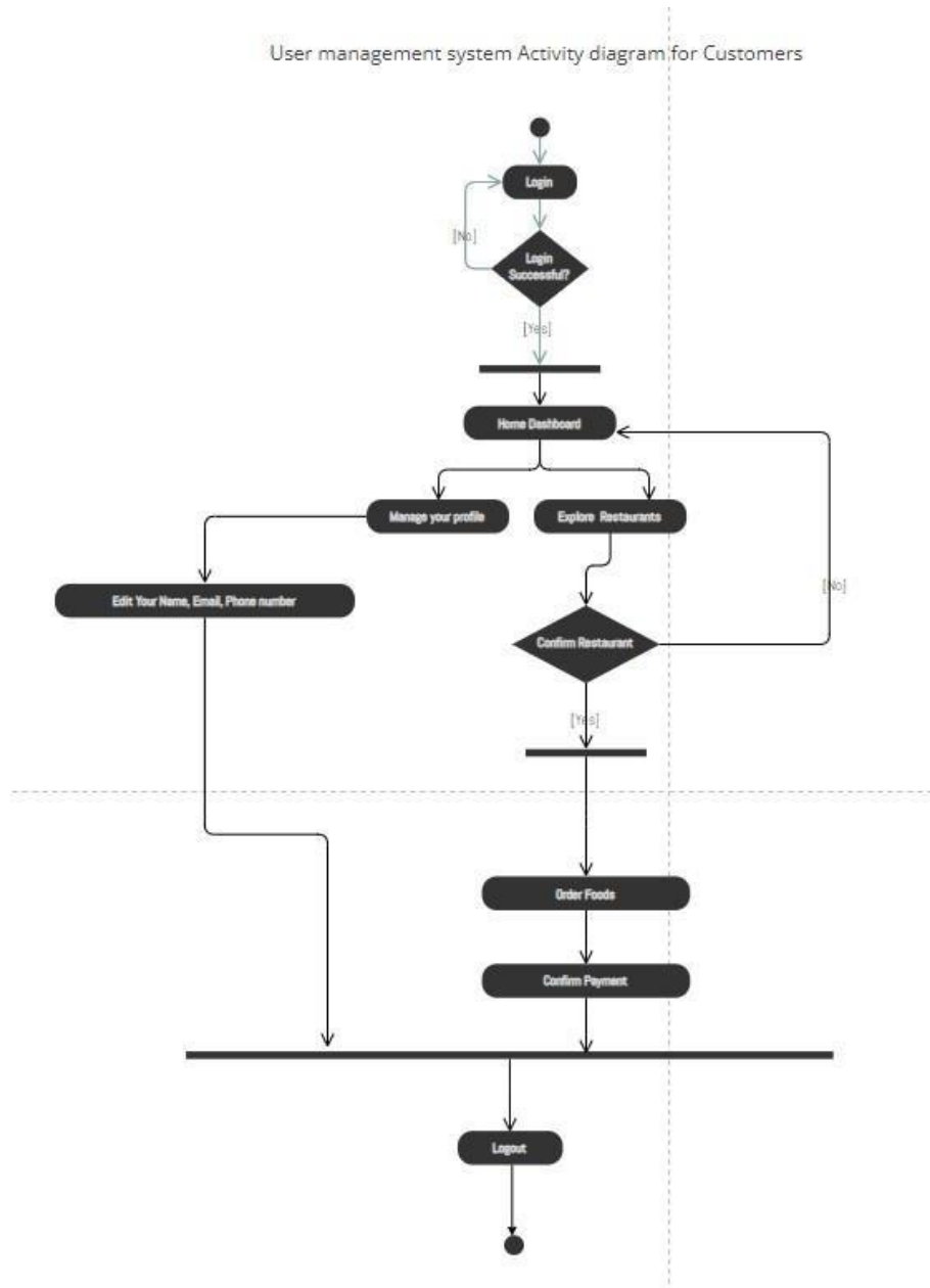
Figure 2 Activity Diagram for Customers UM
