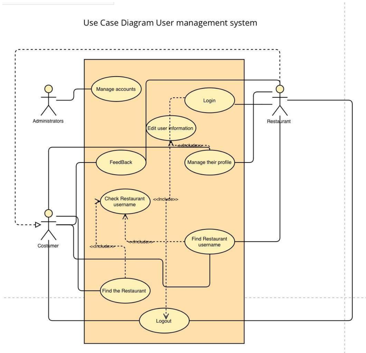
Figure 4 Use Case Diagram User management system
