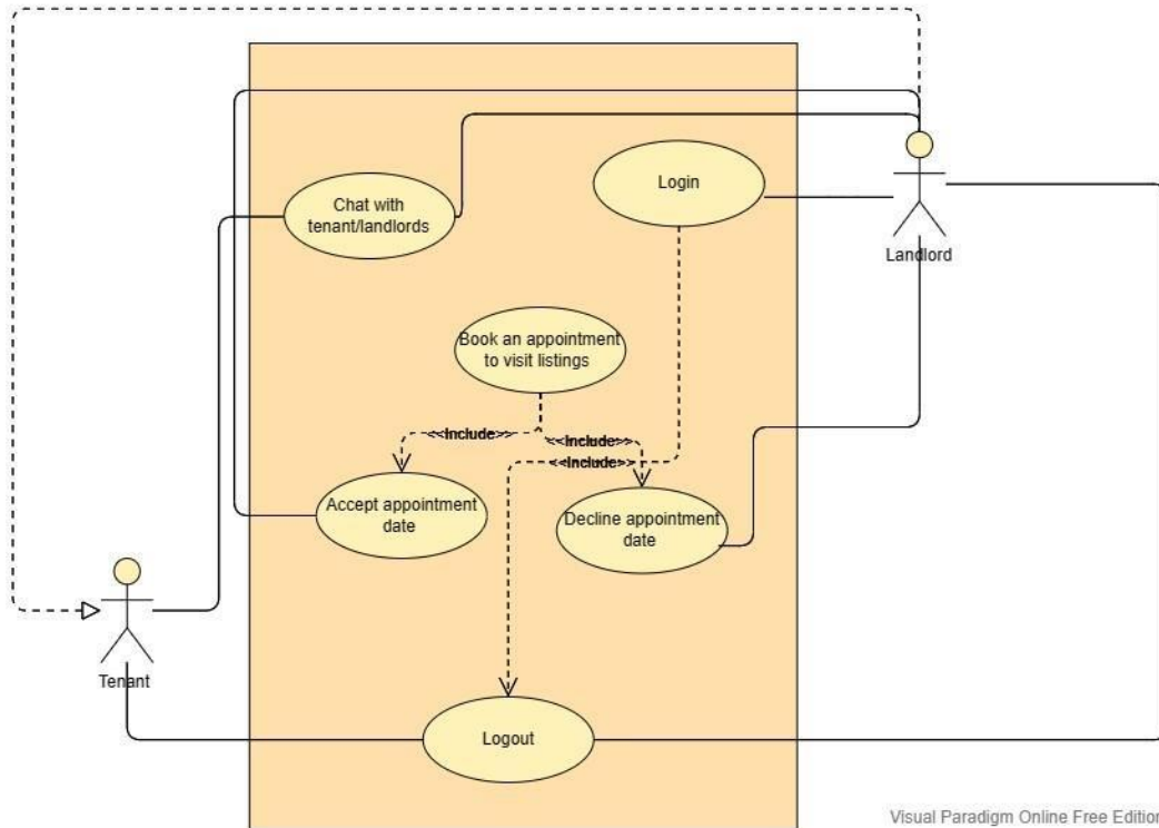
Figure 14 Use Case Diagram OM
