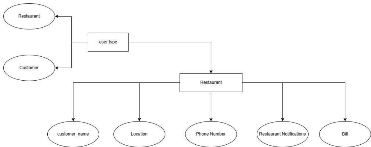
Figure 19 ERD RM
