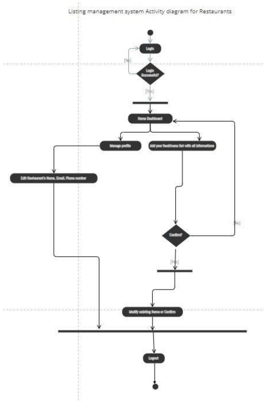
Figure 8 Activity Diagram for Restaurants LM
