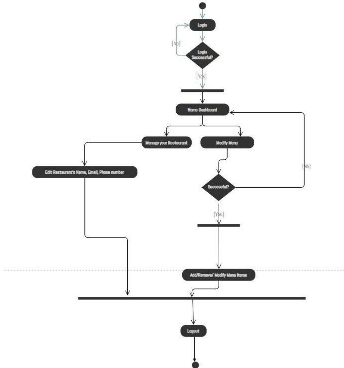
Figure 3 Activity Diagram for Restaurants UM
