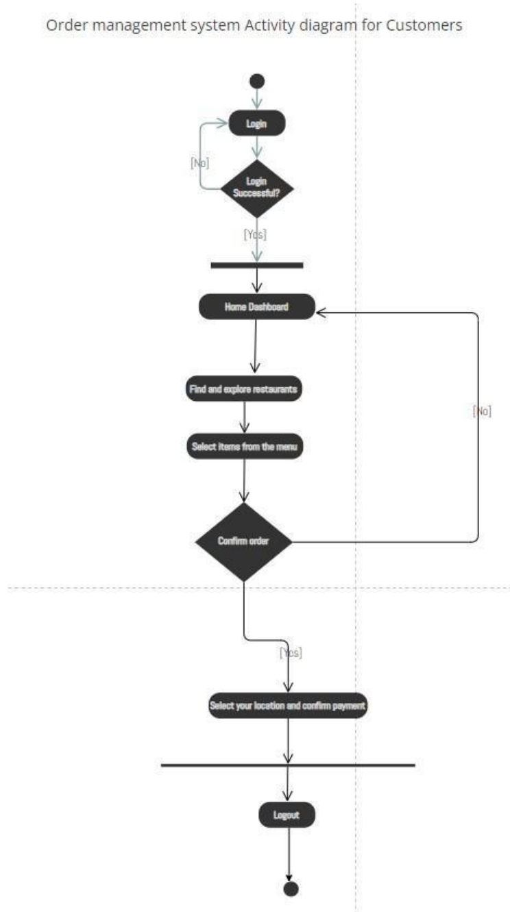
Figure 12 Activity Diagram customer OM
