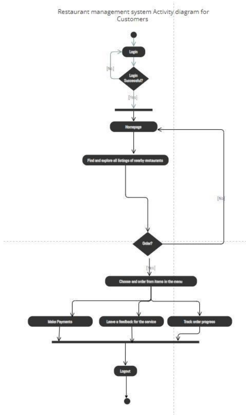
Figure 16 Activity Diagram Customer RM
