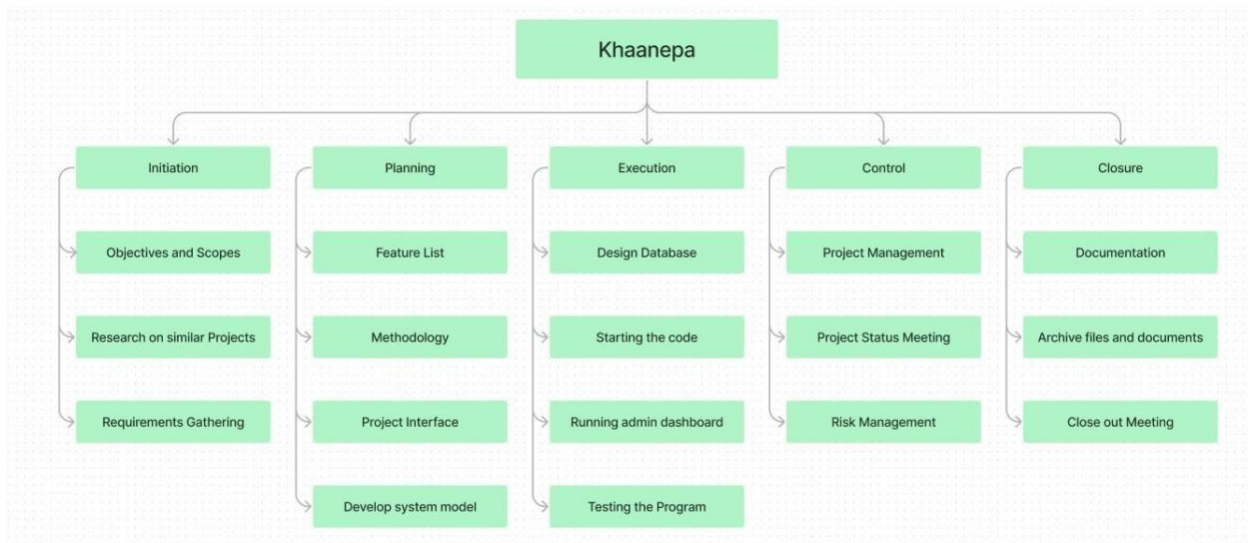
Figure 1 WBS
