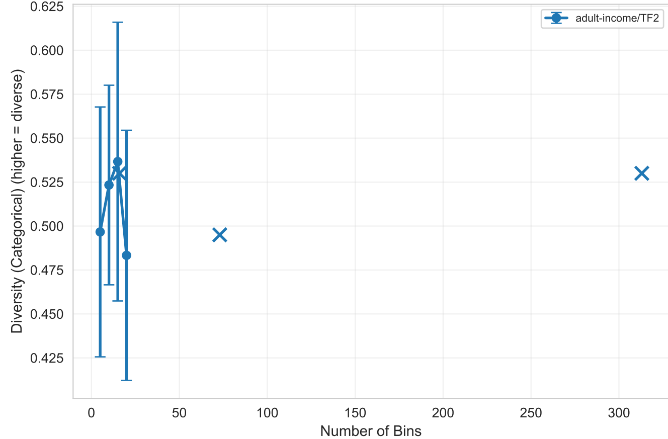
Diversity (Categorical)
