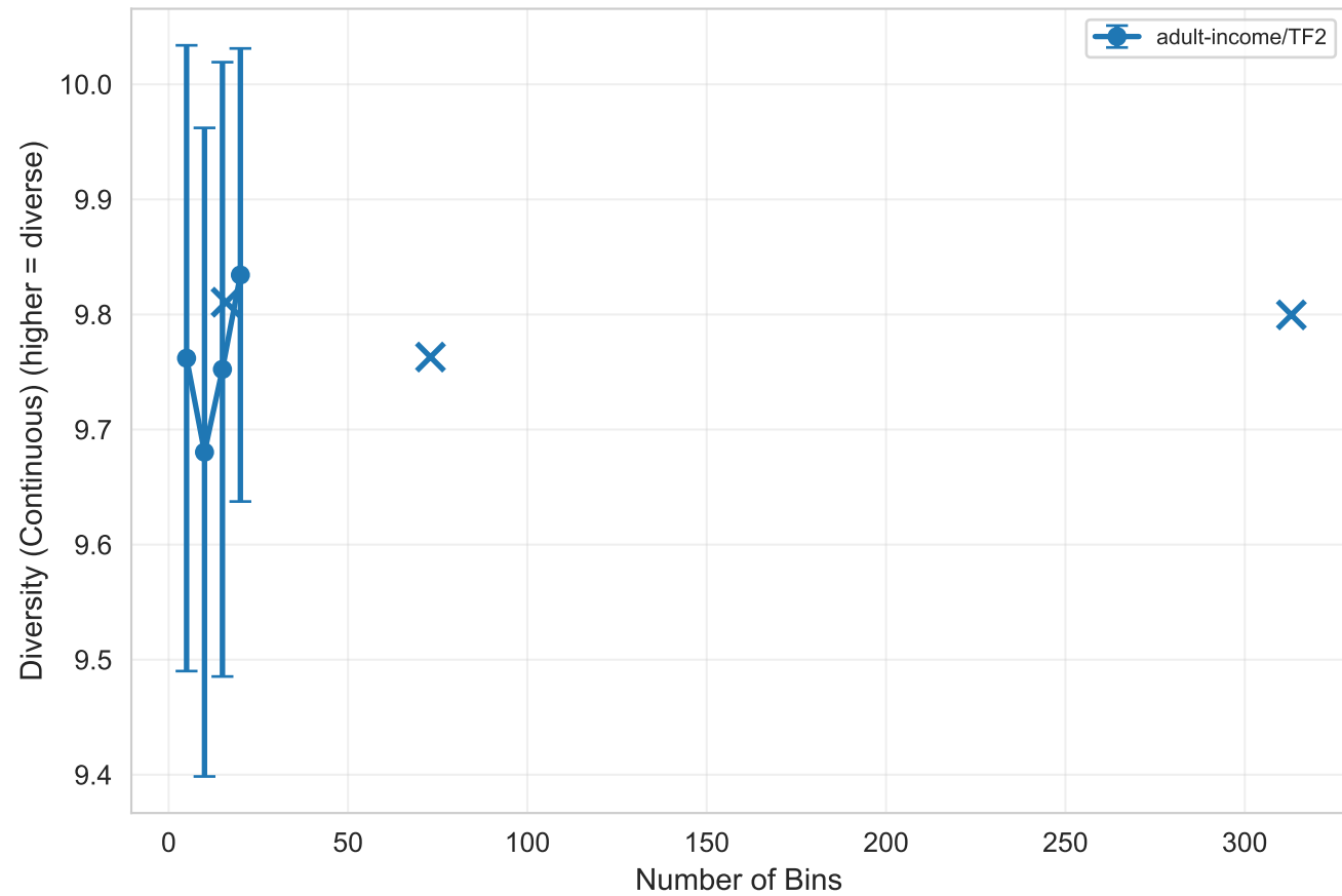
Diversity (Continuous)
