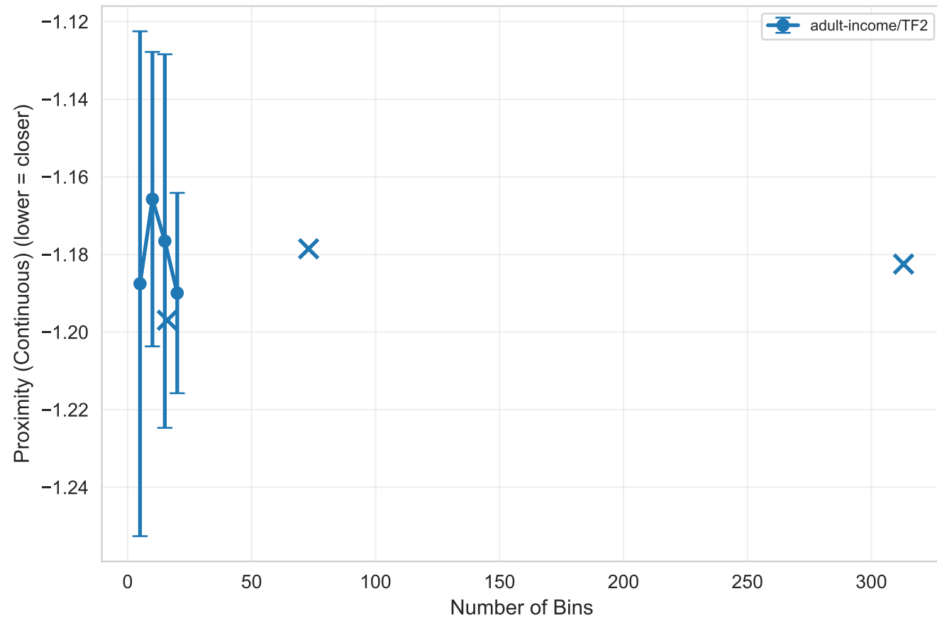
Proximity (Continuous)
