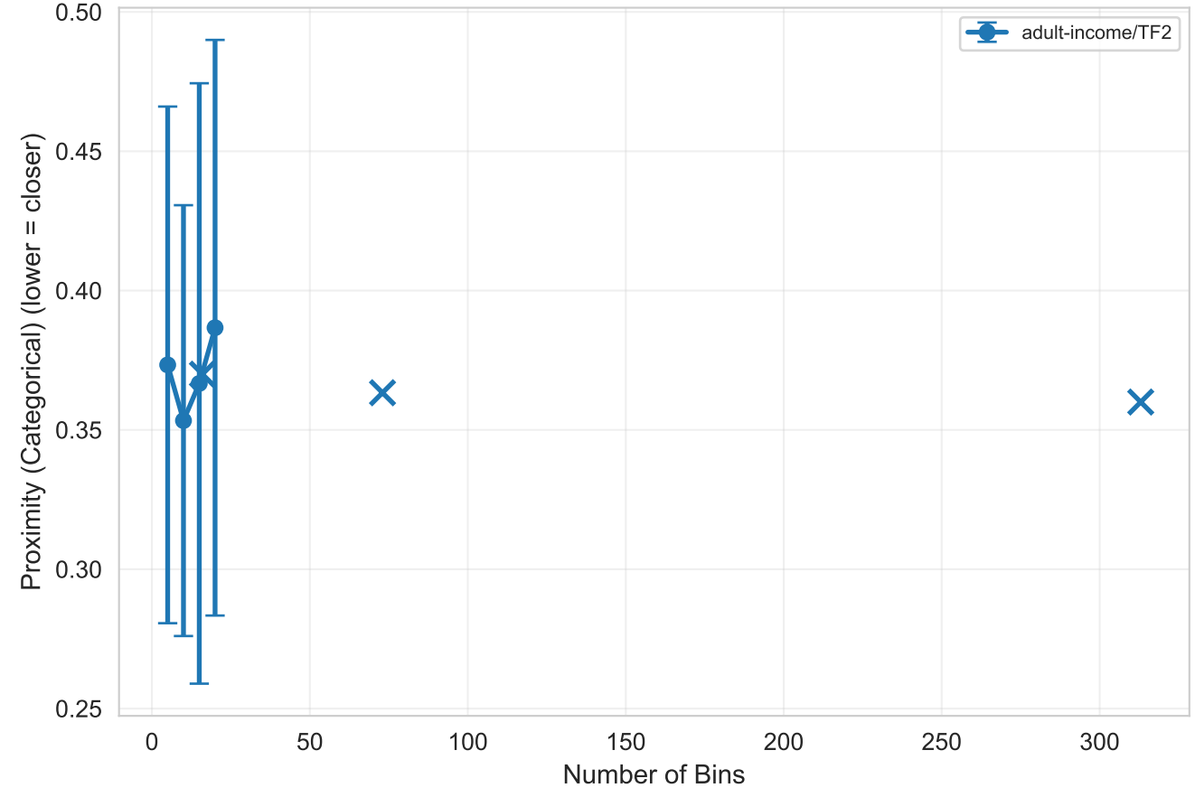
Proximity (Categorical)
