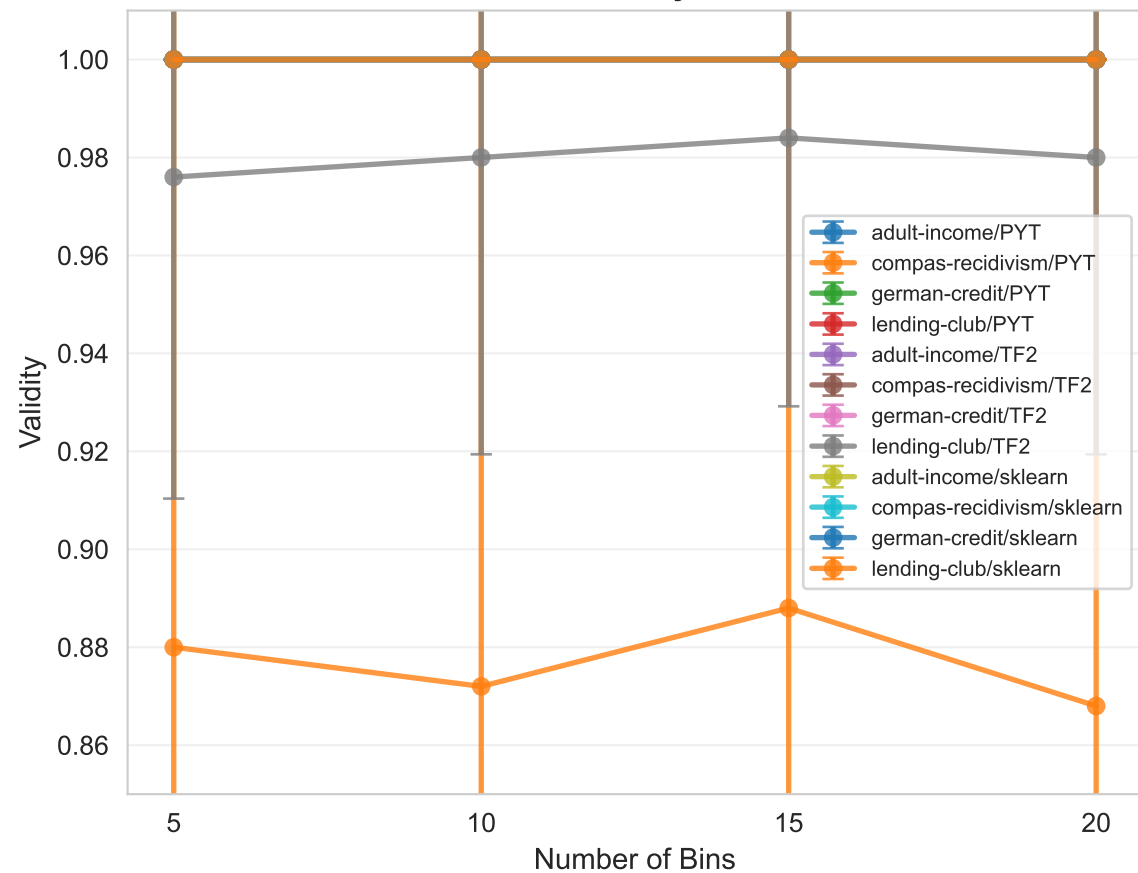
Validity
