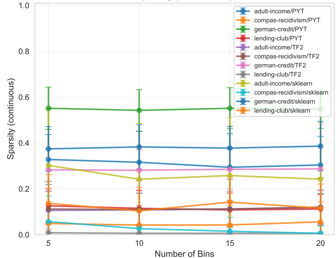
Sparsity (continuous)
