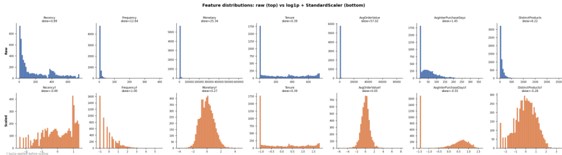
Figure 4.2 Feature distributions before (top) and after (bottom) the log1p + standardisation preprocessing.
