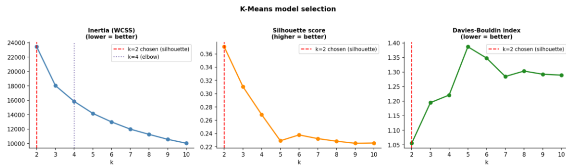
Figure 4.4 K-Means model selection: inertia with the detected elbow (k = 4), silhouette (max at k = 2), and Davies–Bouldin versus k.
