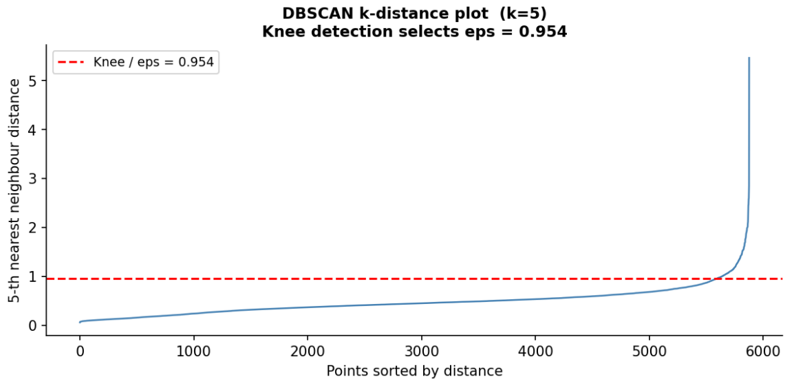
Figure 4.6 DBSCAN k-distance plot; the knee sets the neighbourhood radius \epsilon .
