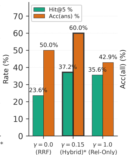
(B) Reranker (N = 50)
