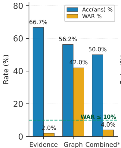
(A) Verification (N = 50)
