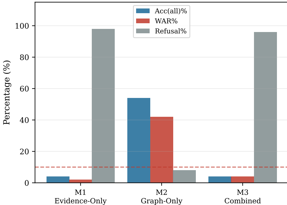
(A) Verification Ablation (N=50)
