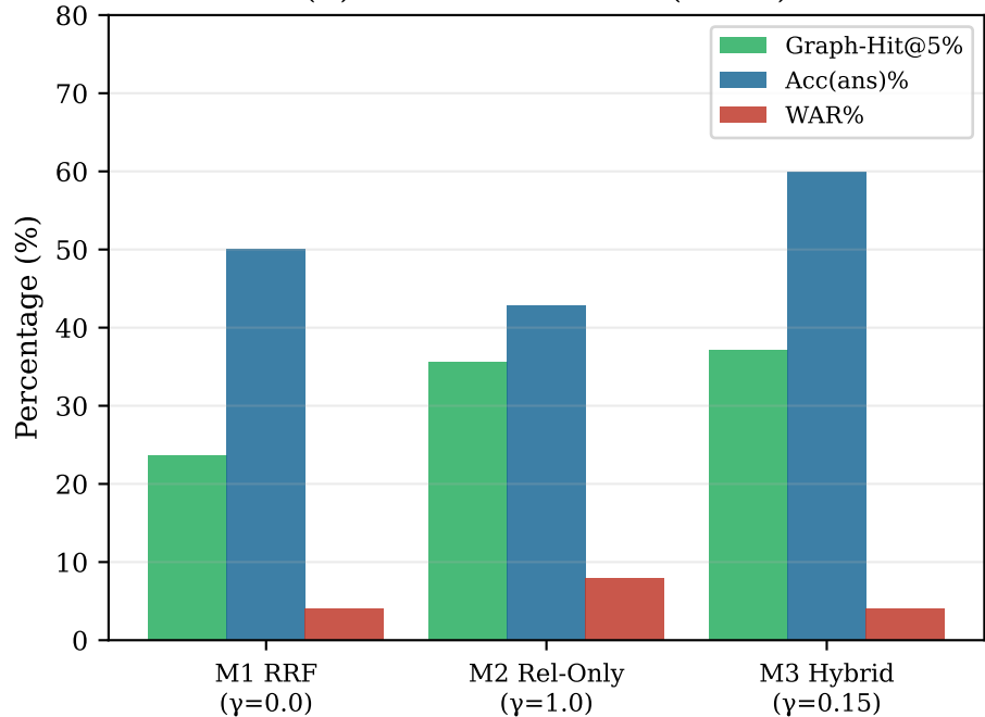
(B) Reranker Ablation (N=50)
