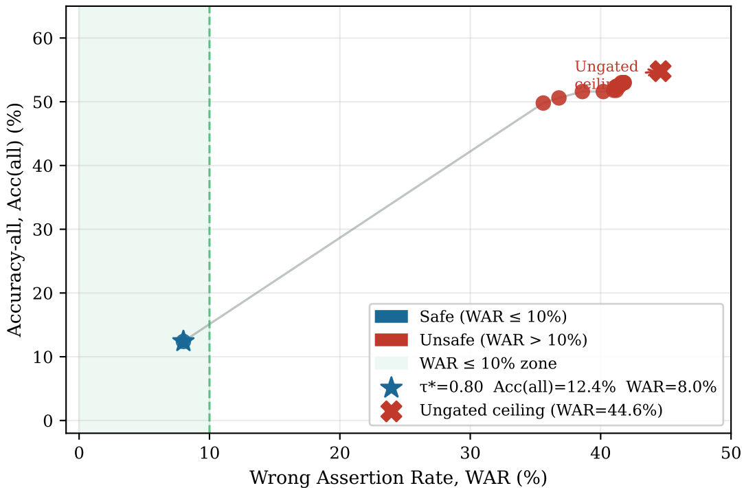
Pareto Frontier: Acc(all) vs WAR — M2 Graph-Only (N=500)
