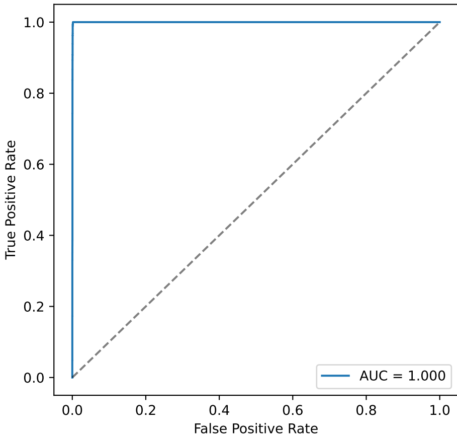
Discriminator ROC - CaloChallenge HLV
