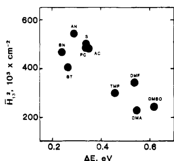
Figure 2. Dependence of \bar{H}_{13}^2 on donor-acceptor separation energy for (\text{bpy})_2\text{ClRu}(\text{pyz})\text{Ru}(\text{NH}_3)_4(\text{pyridine})^{4+} . Key to solvents as in Figure 1.
