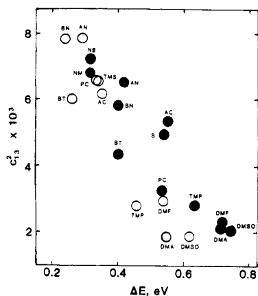
Figure 1. Dependence of c_{13}^2 on separation energy for (○) (\text{bpy})_2\text{ClRu}(\text{pyz})\text{Ru}(\text{NH}_3)_4(\text{pyridine})^{4+} and (●) (\text{bpy})_2\text{ClRu}(\text{pyz})\text{Ru}(\text{NH}_3)_5^{4+} . Key to solvents: NM = nitromethane, NB = nitrobenzene, BN = benzonitrile, AN = acetonitrile, S = sulfolane, PC = propylene carbonate, BT = butyronitrile, AC = acetone, TMP = trimethyl phosphate, DMF = dimethylformamide, DMA = dimethylacetamide, DMSO = dimethyl sulfoxide.
