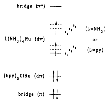
Figure 3. Molecular orbital diagrams for (\text{bpy})_2\text{ClRu}^{\text{II}}(\text{pyz})\text{Ru}^{\text{III}}(\text{NH}_3)_4(\text{pyridine})^{4+} and (\text{bpy})_2\text{ClRu}^{\text{II}}(\text{pyz})\text{Ru}^{\text{III}}(\text{NH}_3)_5^{4+} in three solvents.
