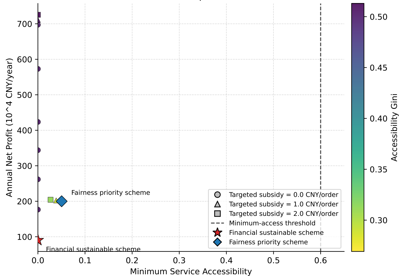
RQ3 Fairness Threshold Gap on the Pareto Frontier
