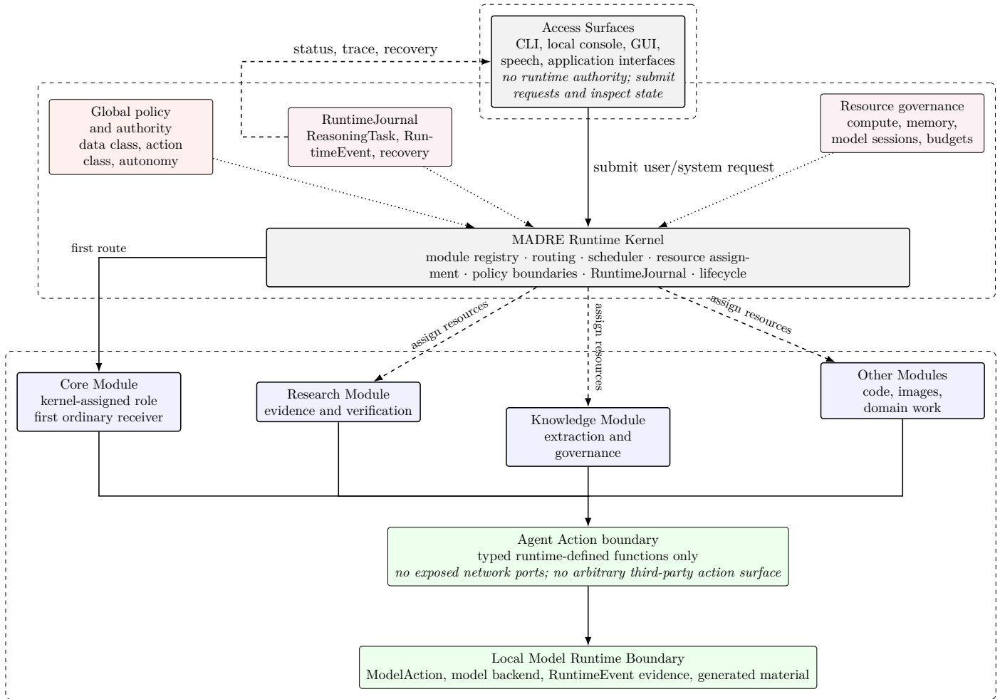
Figure 11.1: MADRE responsibility layers: kernel coordination, Core Module assignment, runtime journal, actions, and inference.
