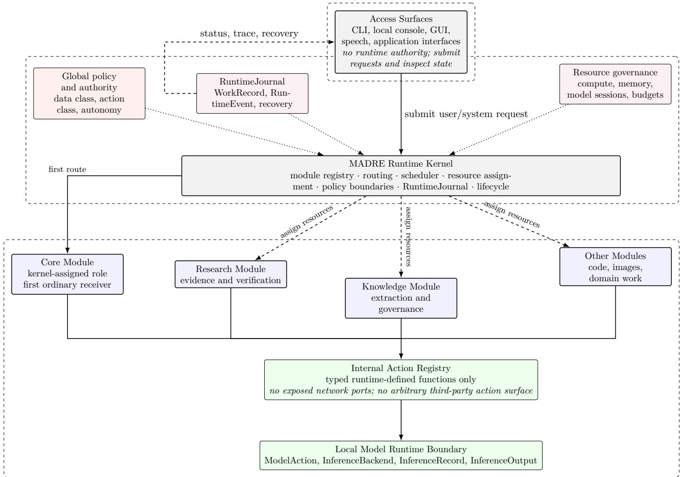
Figure 5.1: MADRE responsibility layers: kernel coordination, Core Module assignment, runtime journal, actions, and inference.
