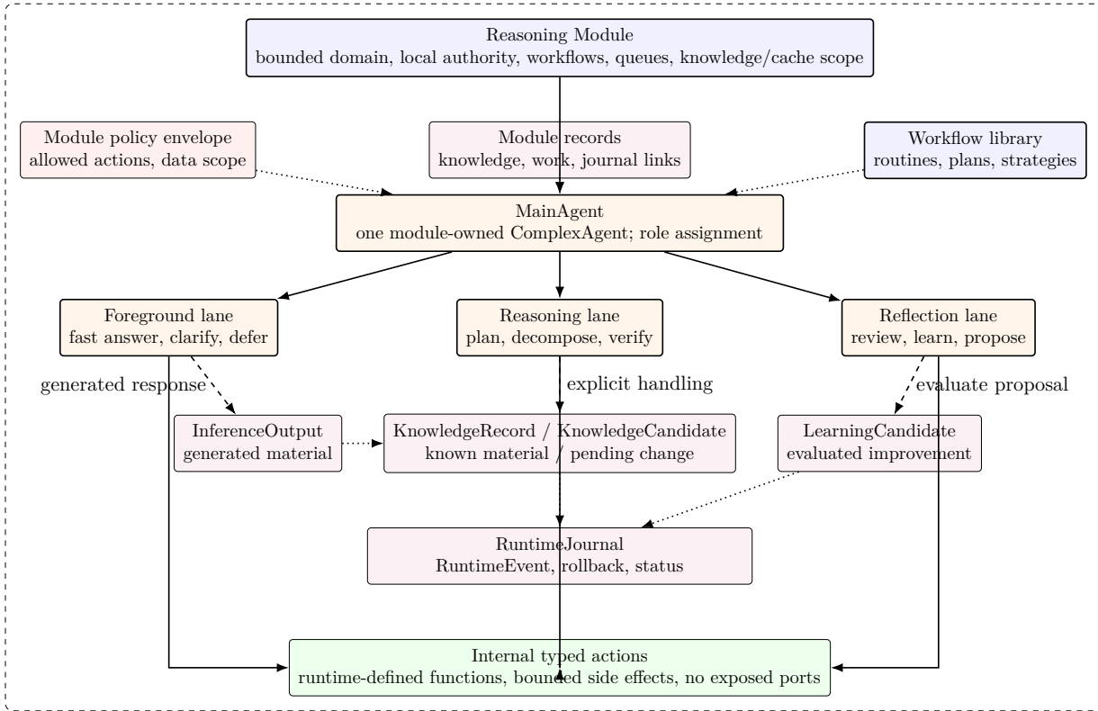
Figure 5.2: Reasoning module internal structure with its MainAgent using a ComplexAgent lane profile.
