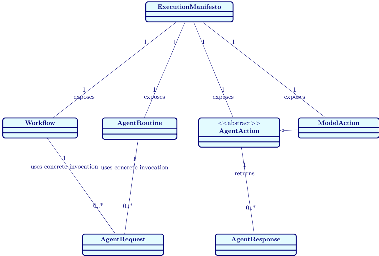
Figure E.7: Reusable capabilities expose manifesto metadata without owning plan-specific scheduling semantics.
