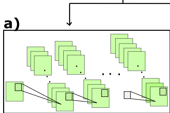
ResNet50
