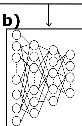
DNN
