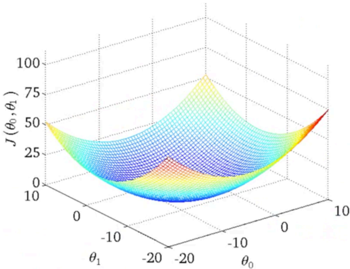
Figure: Visualisation of how the cost function actually depends on two parameters, and the global minimum of the cost for this univariate regression is defined by two parameters.
