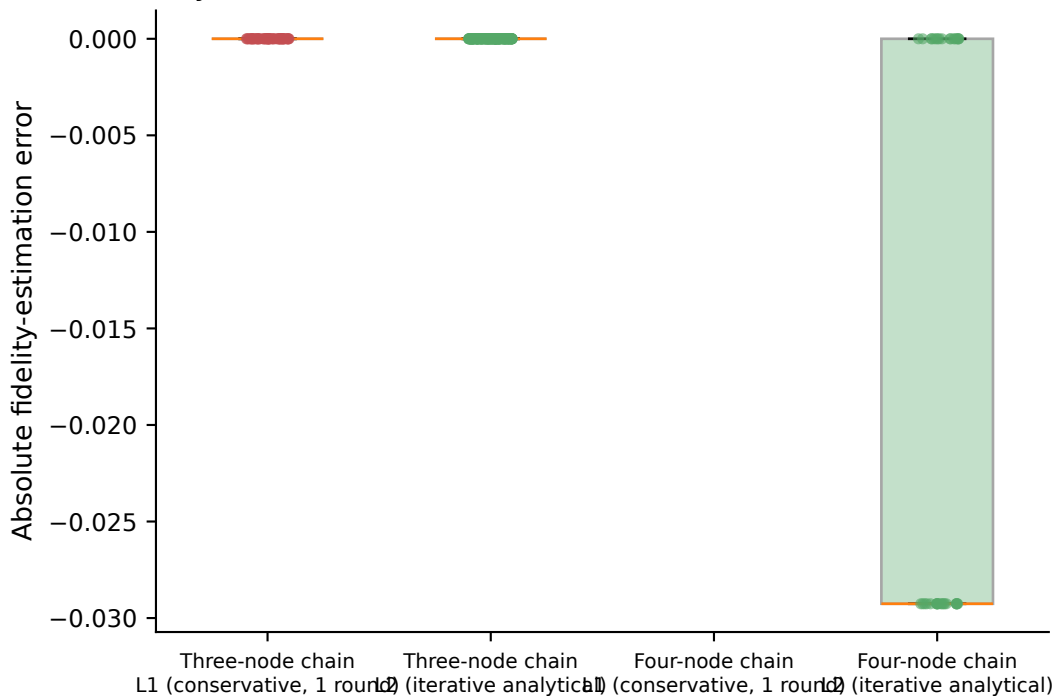
Fidelity-estimation error: L1 vs. L2 (SATISFIED/VIOLATED trials only)
