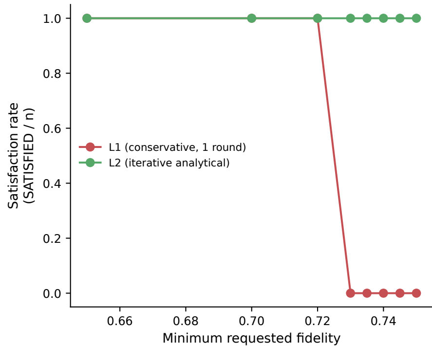
Three-node chain
