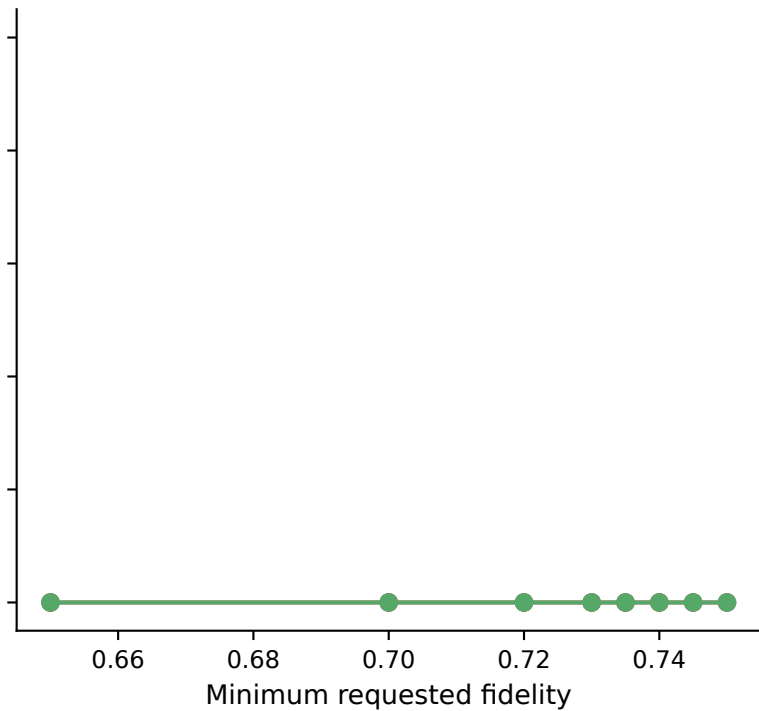
Four-node chain
