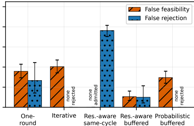
Ideal local operations
