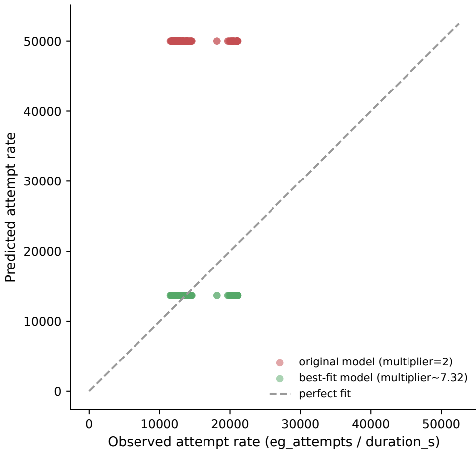
L3 attempt-rate audit: predicted vs. observed
