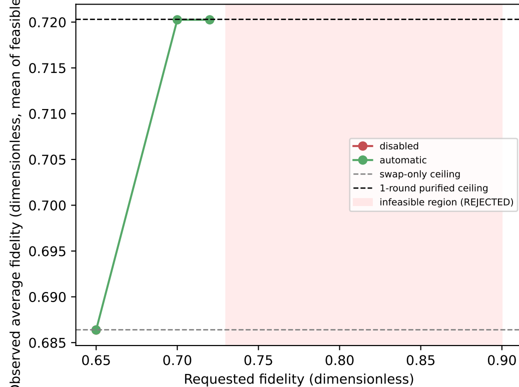
Requested vs. observed fidelity
