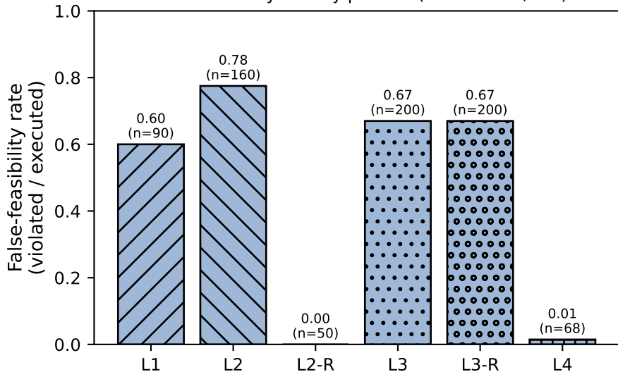
False-feasibility rate by planner (P02b + P03/P13)
