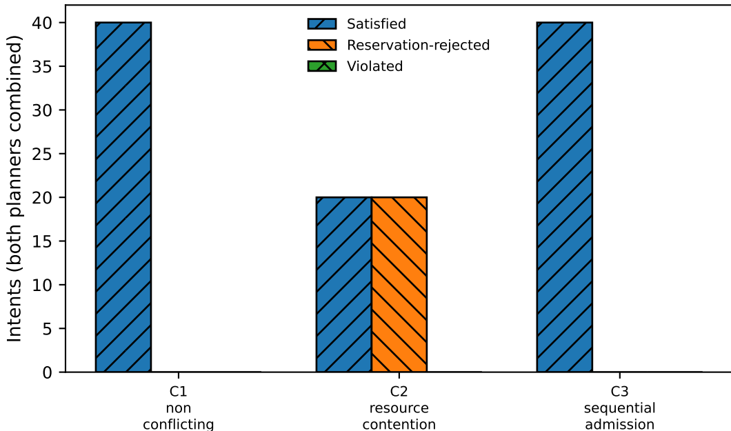
Multi-intent outcomes by scenario (P17, 40 intents/scenario) Admission (planner) vs. reservation rejection (NetworkManager) vs. final outcome
