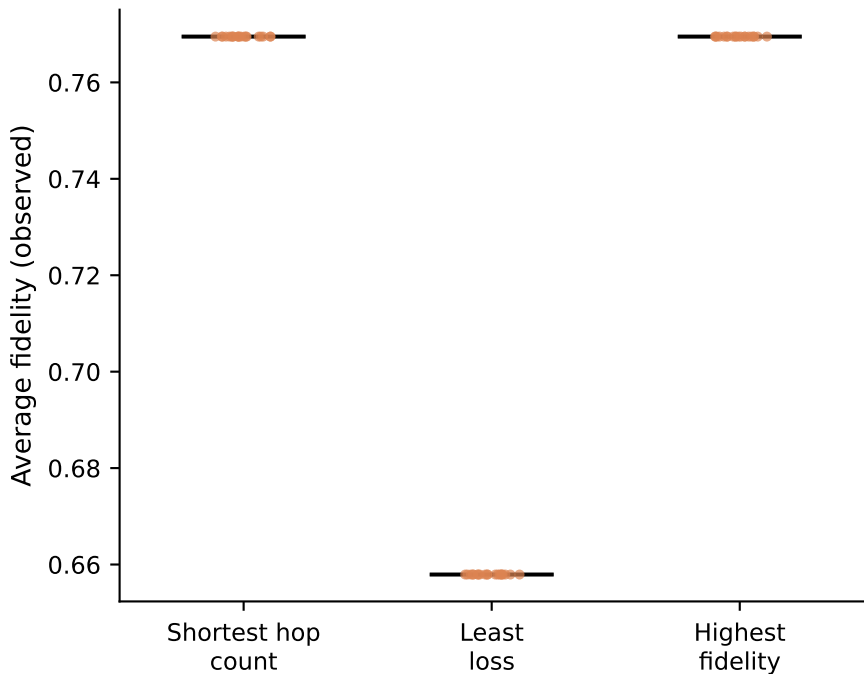
Observed fidelity under alternative routing strategies (diamond heterogeneous)
