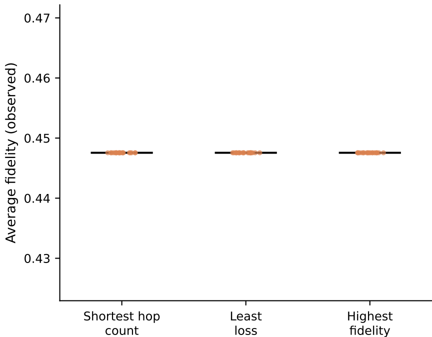
Observed fidelity under alternative routing strategies (small mesh)
