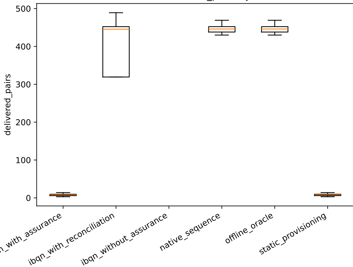
F01 architecture/baselines - delivered_pairs by condition (n=20 seeds)
