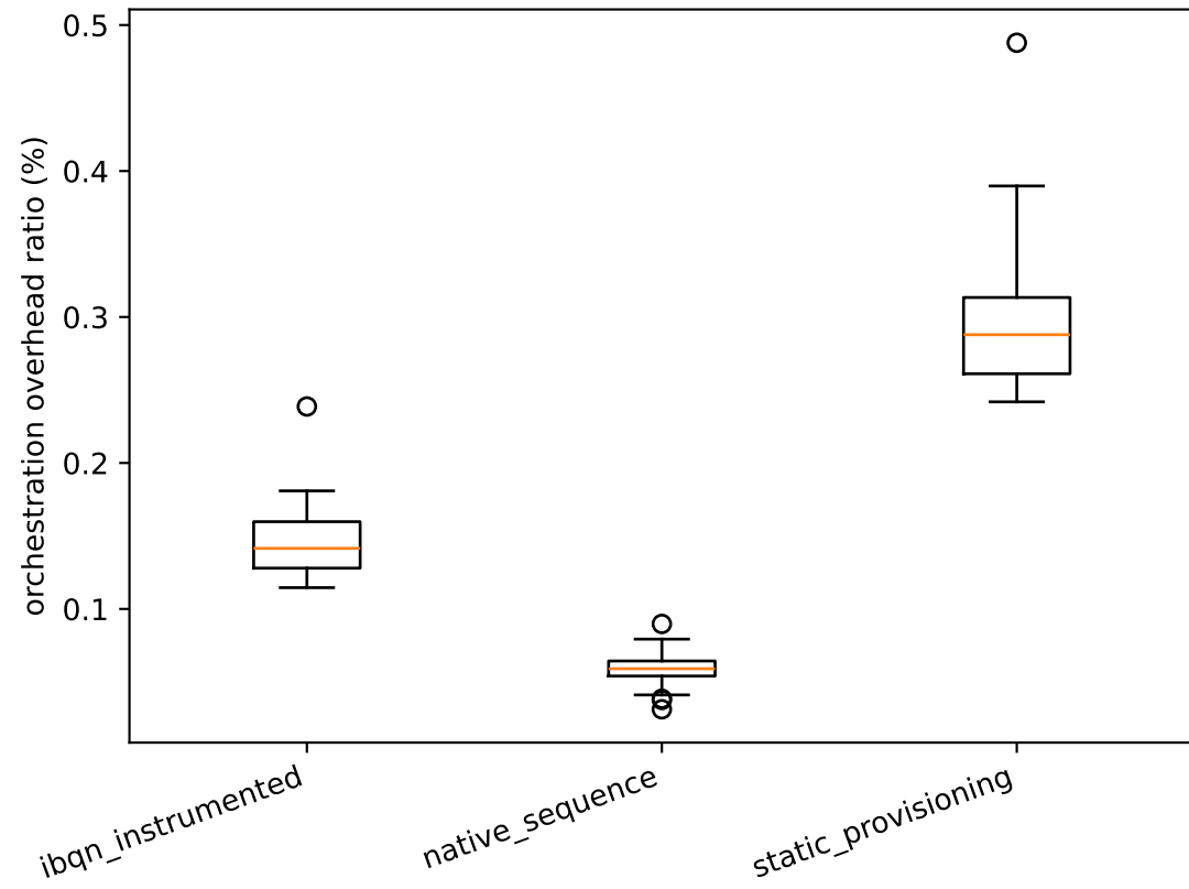
F06 overhead - distribution by condition (n=20 seeds)
