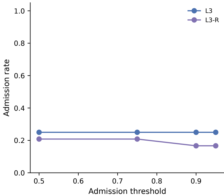
(A) Does the threshold change decisions?
