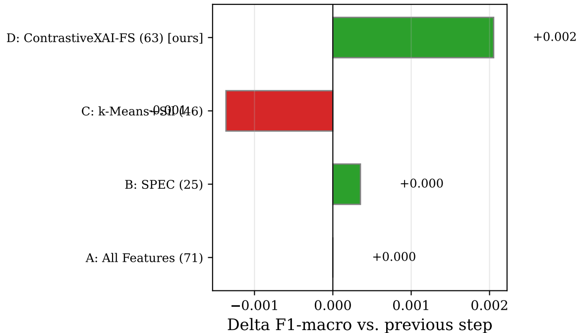
Incremental Gain per Component (Binary Classification (label1))
