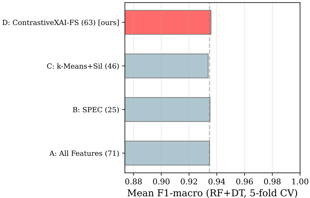
F1-macro by Configuration (Binary Classification (label1))
