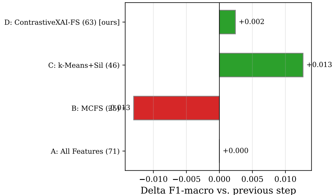
Incremental Gain per Component (8-Class Attack Classification (label2))
