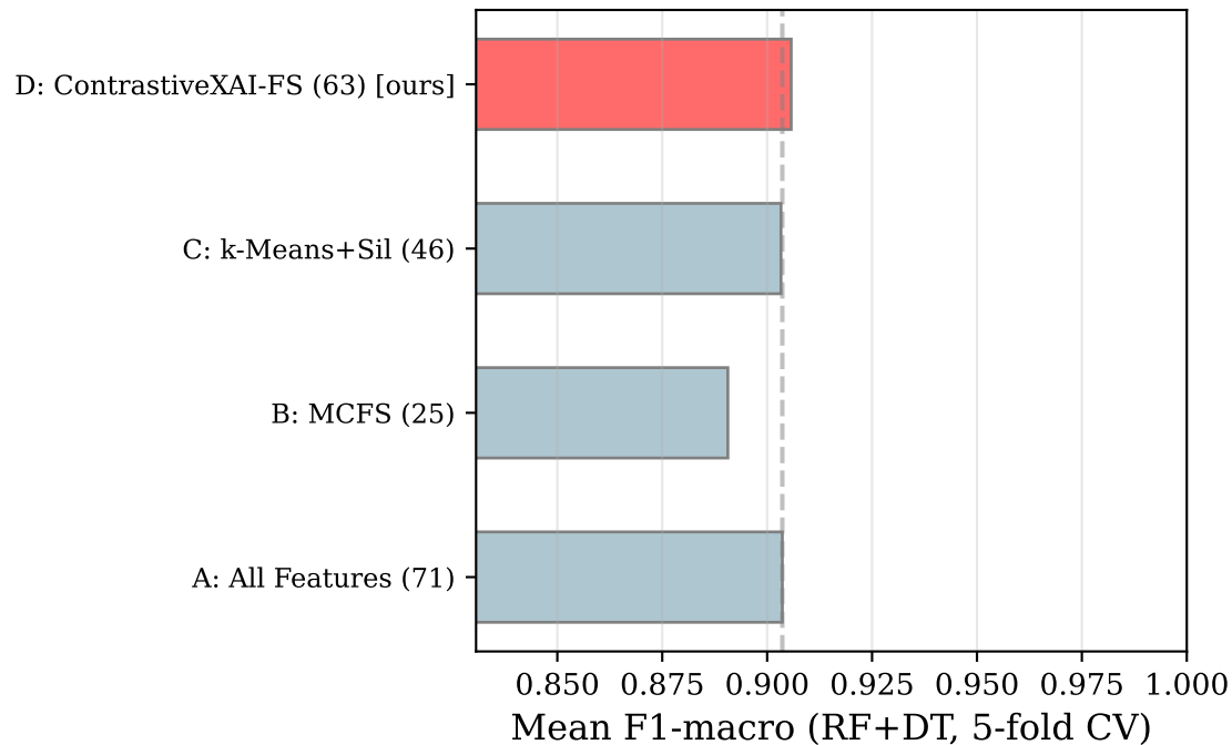
F1-macro by Configuration (8-Class Attack Classification (label2))
