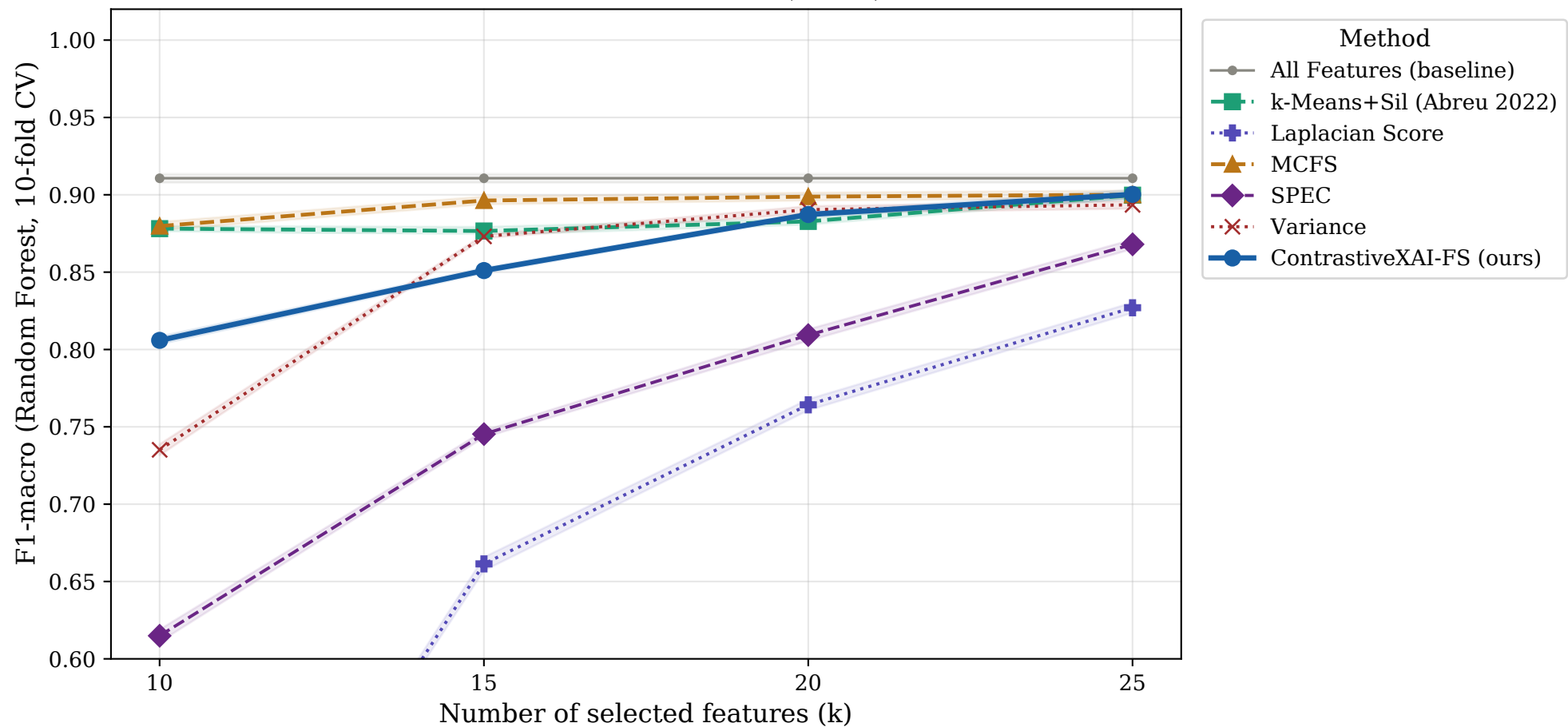
8-Class Attack Classification (label2)
