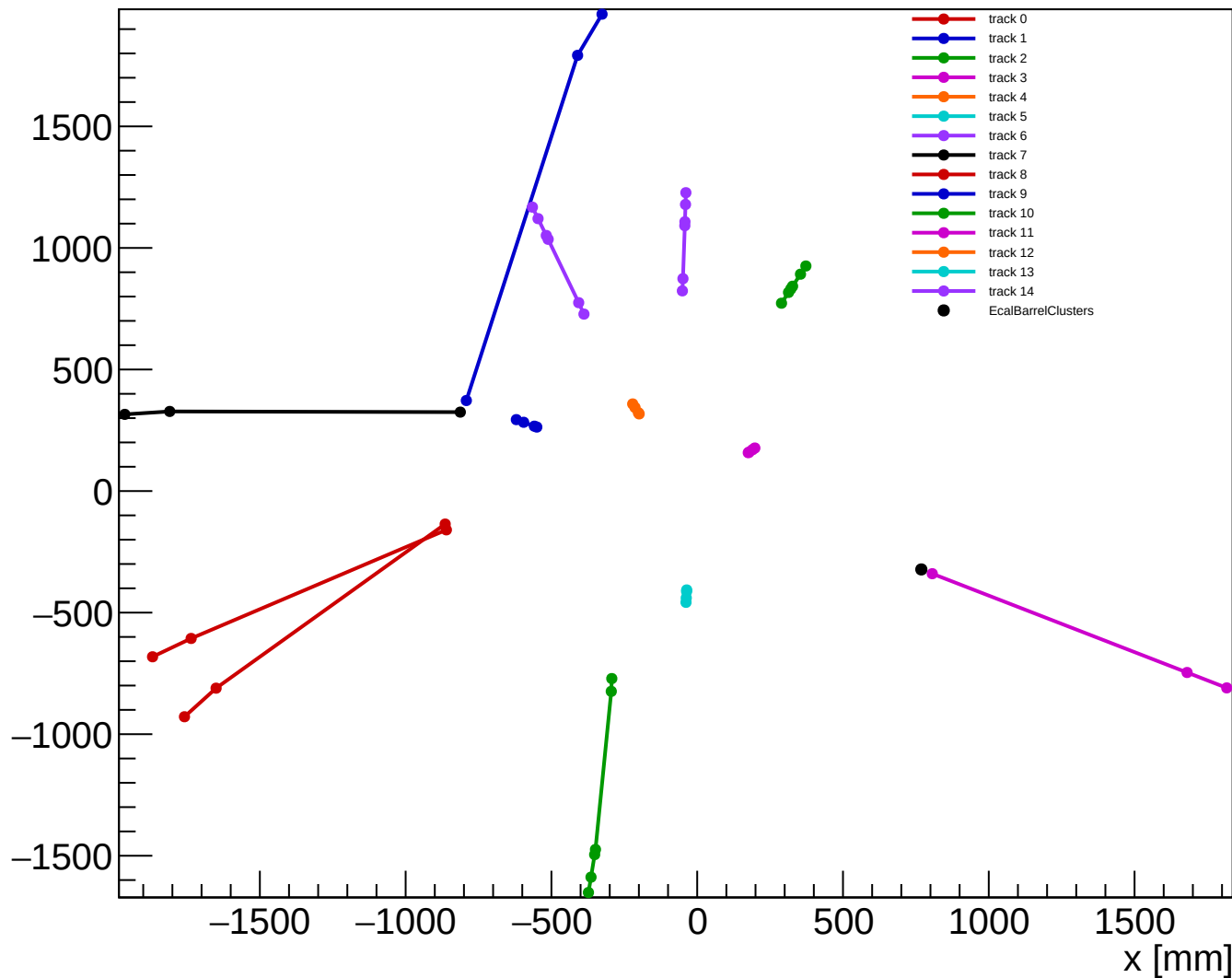
Event 2 track projection points and ECal clusters
