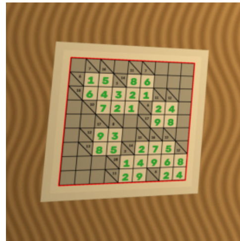
✓ 08_photo_warm
