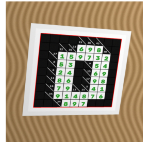
✓ 10_photo_rotated
