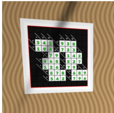
✓ 12_scan_navy
