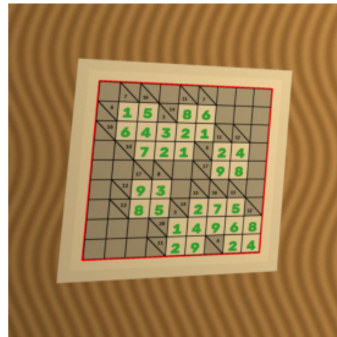
✓ 08_photo_warm
