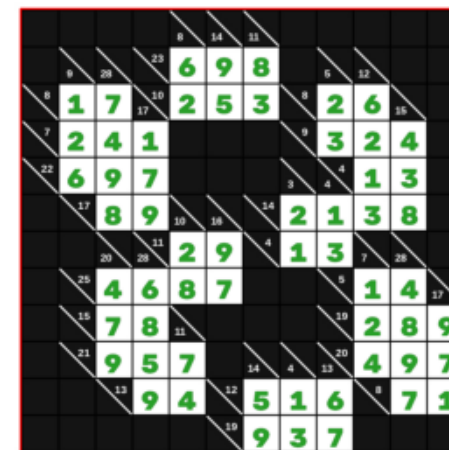
✓ 14_large_digital
