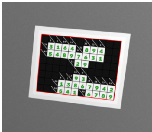
✓ 13_rect_photo
