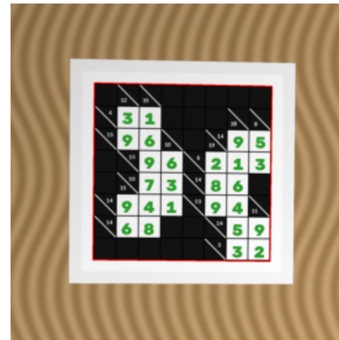
✓ 09_photo_blur
