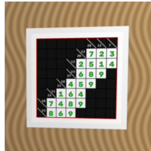
✓ 14_large_digital
