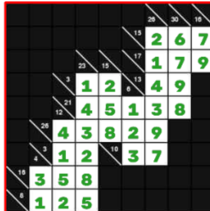
✓ 08_photo_warm
