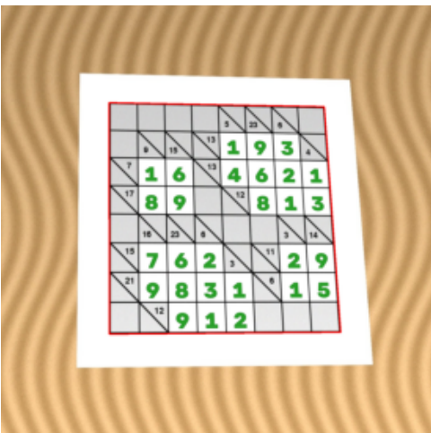
✓ 11_photo_overexp
