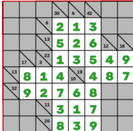
✓ 07_photo_shadow
