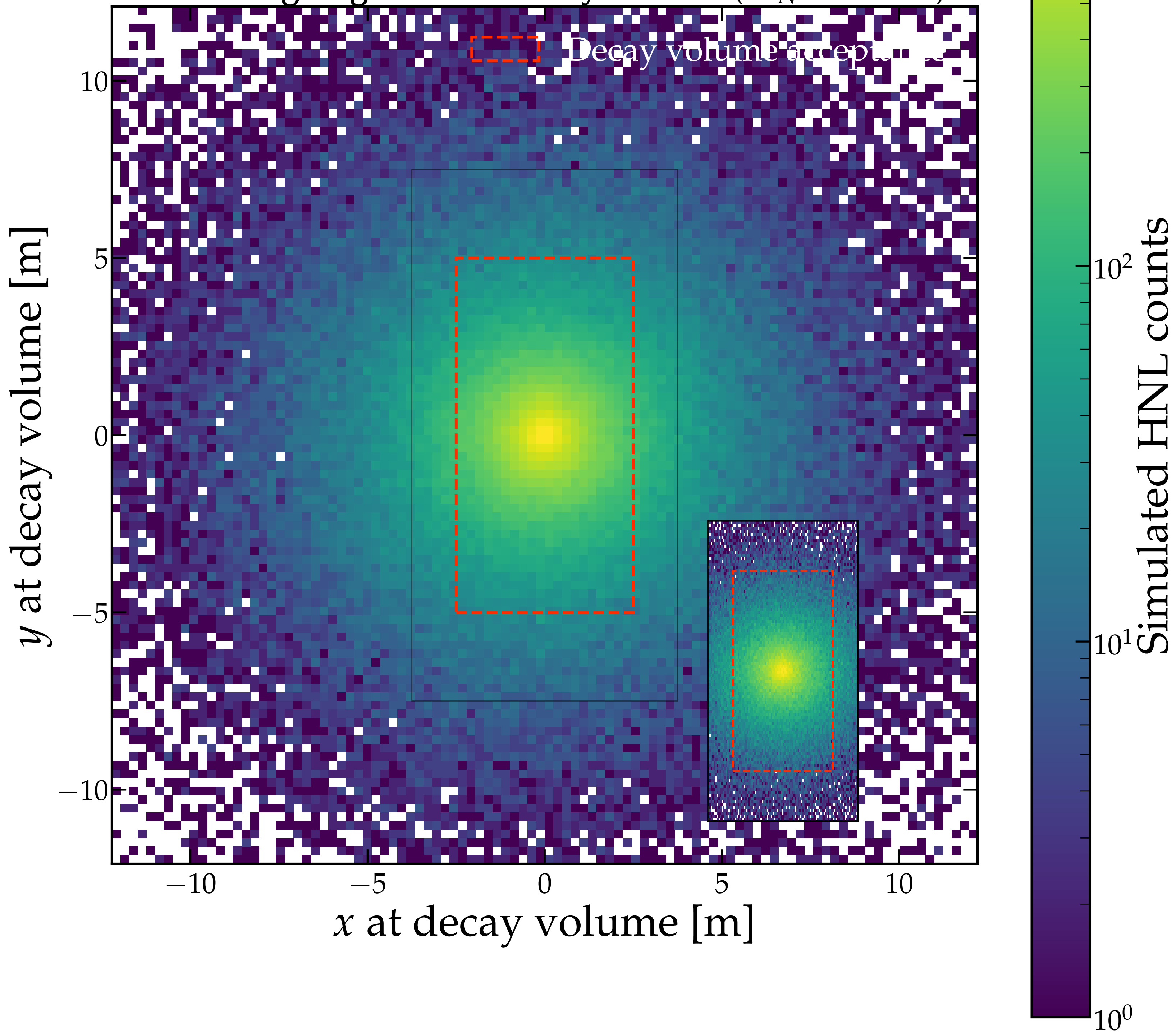
Forward-going HNLs at decay volume ( M_N = 1 GeV)
