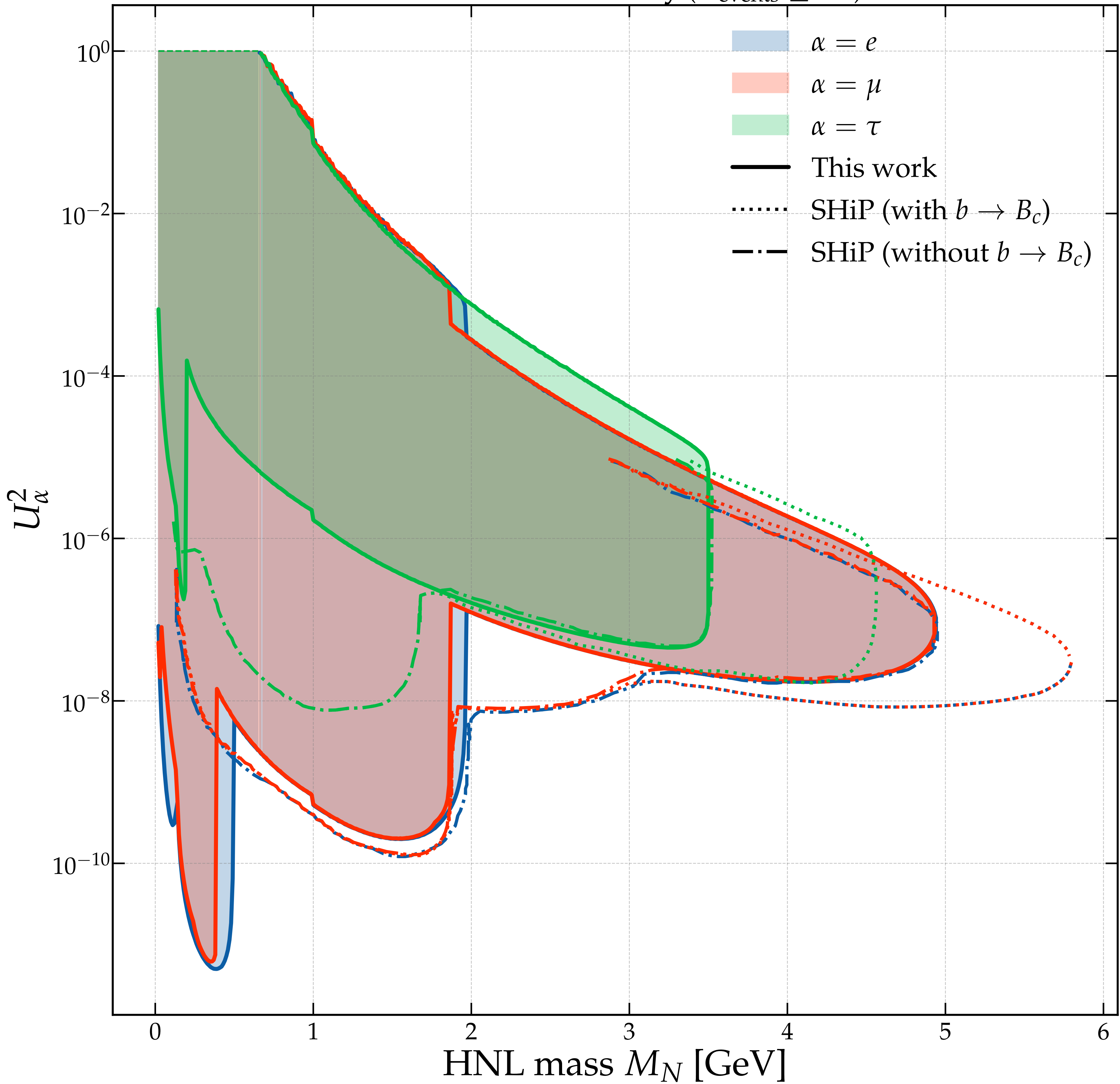
SHiP 90% CL sensitivity ( \bar{N}_{\text{events}} \geq 2.3 )
