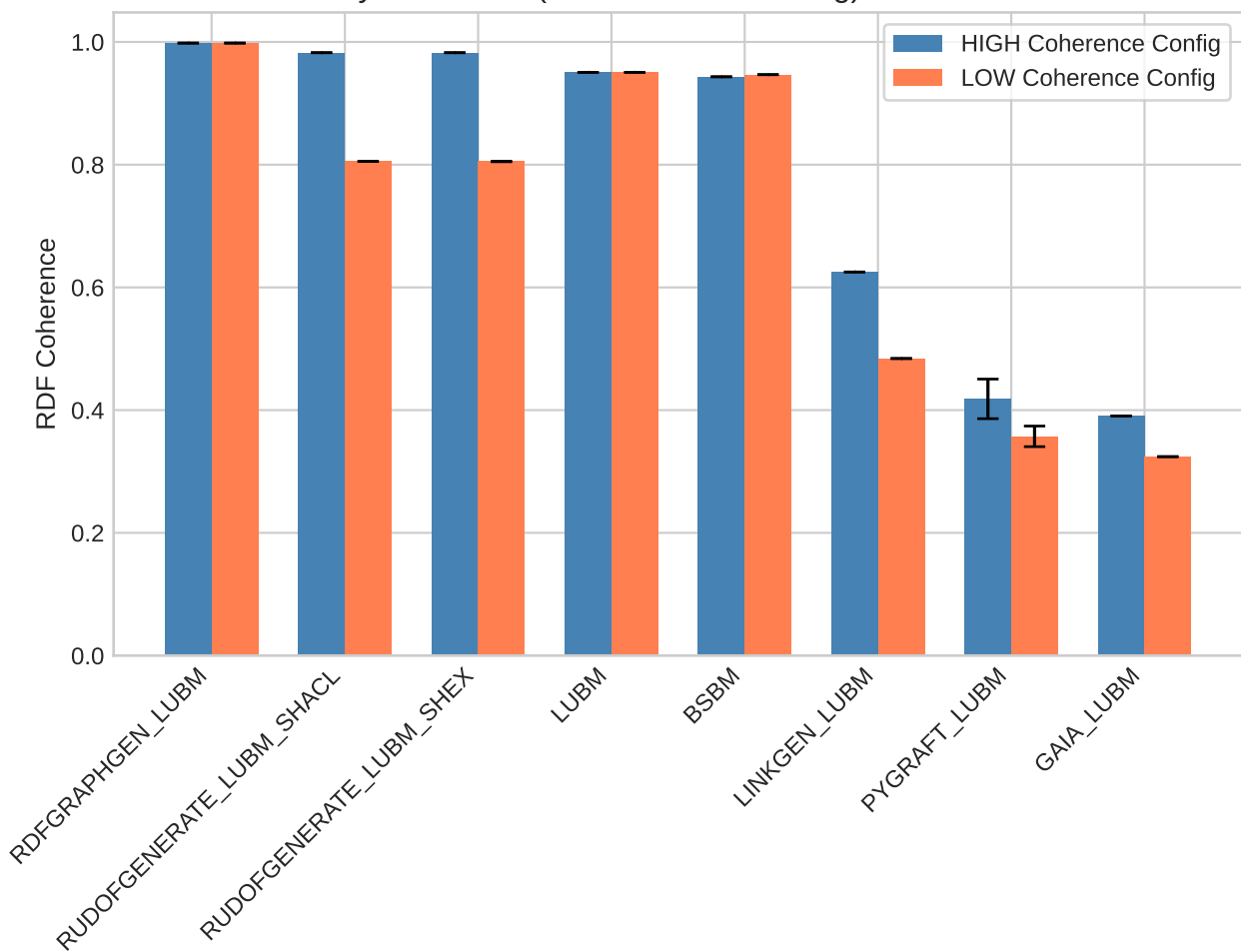
RDF Coherence by Generator (HIGH vs LOW Config) — mean \pm std over 10 runs
