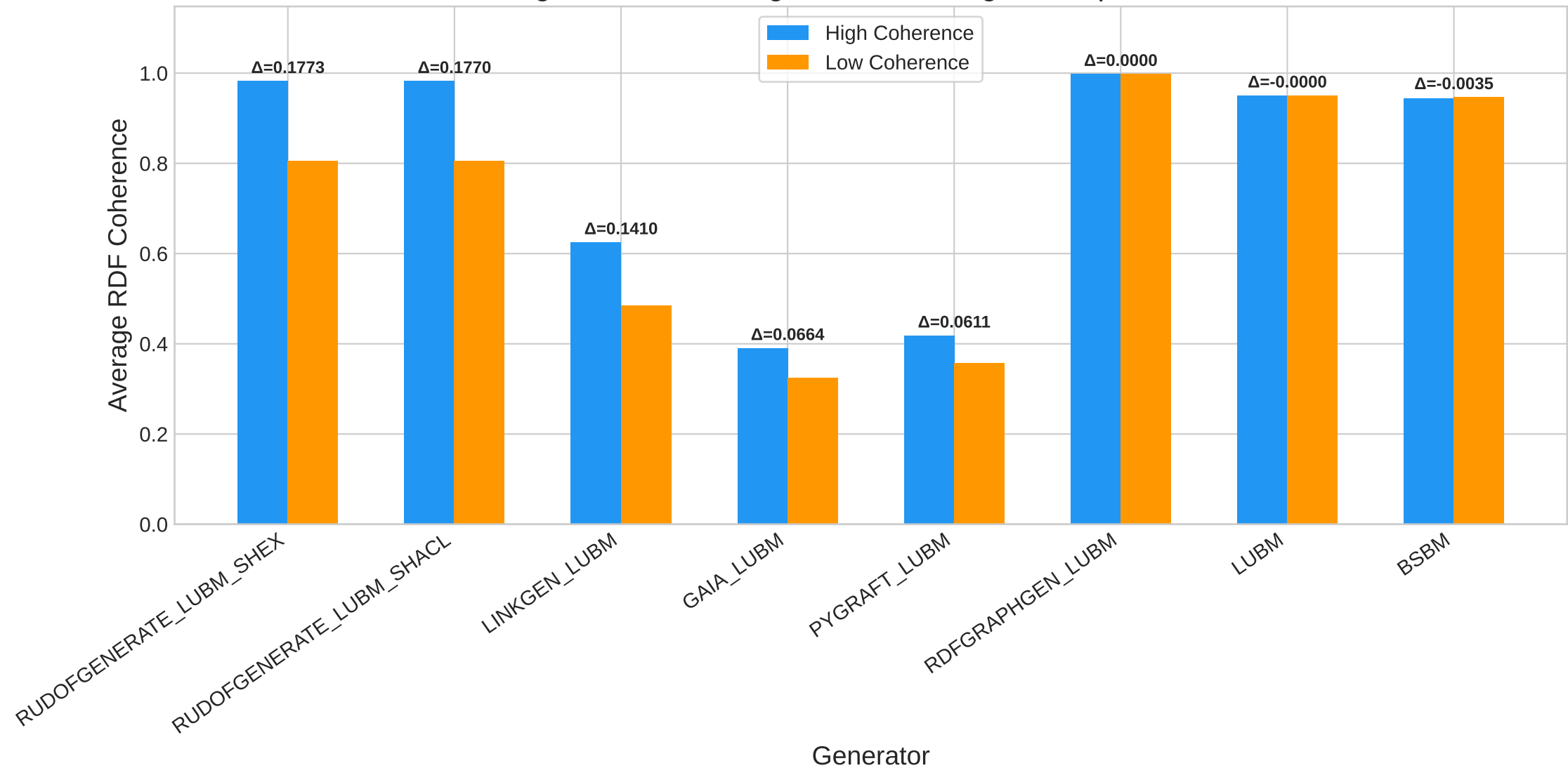
Average Coherence: High vs Low Configuration per Generator
