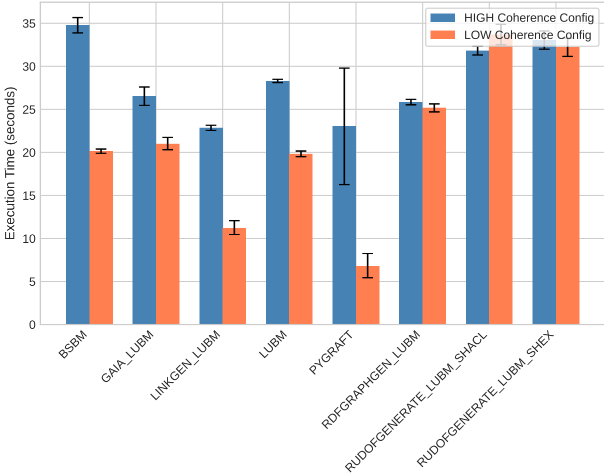
Execution Time by Generator (HIGH vs LOW Config) — mean \pm std over 10 runs
