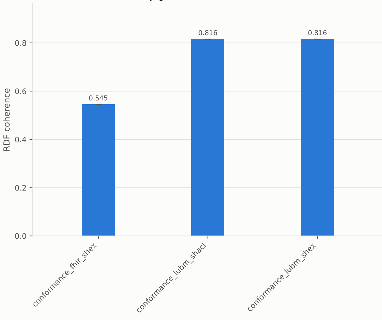
RDF coherence by generator - mean \pm std over 3 run(s)
