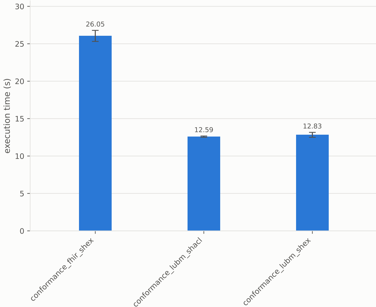
Execution time by generator - mean \pm std over 3 run(s)
