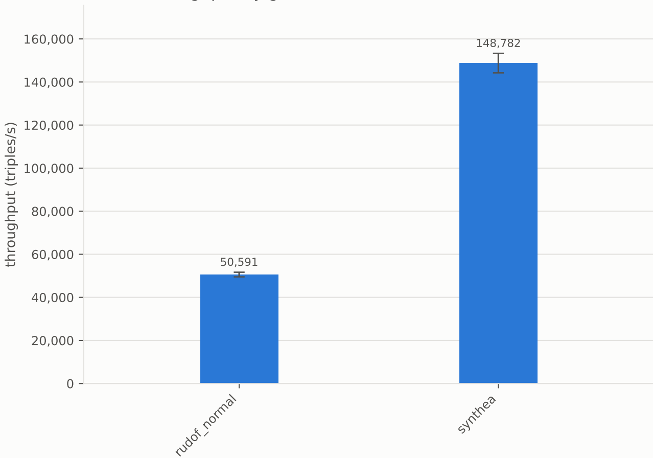
Throughput by generator - mean \pm std over 10 run(s)
