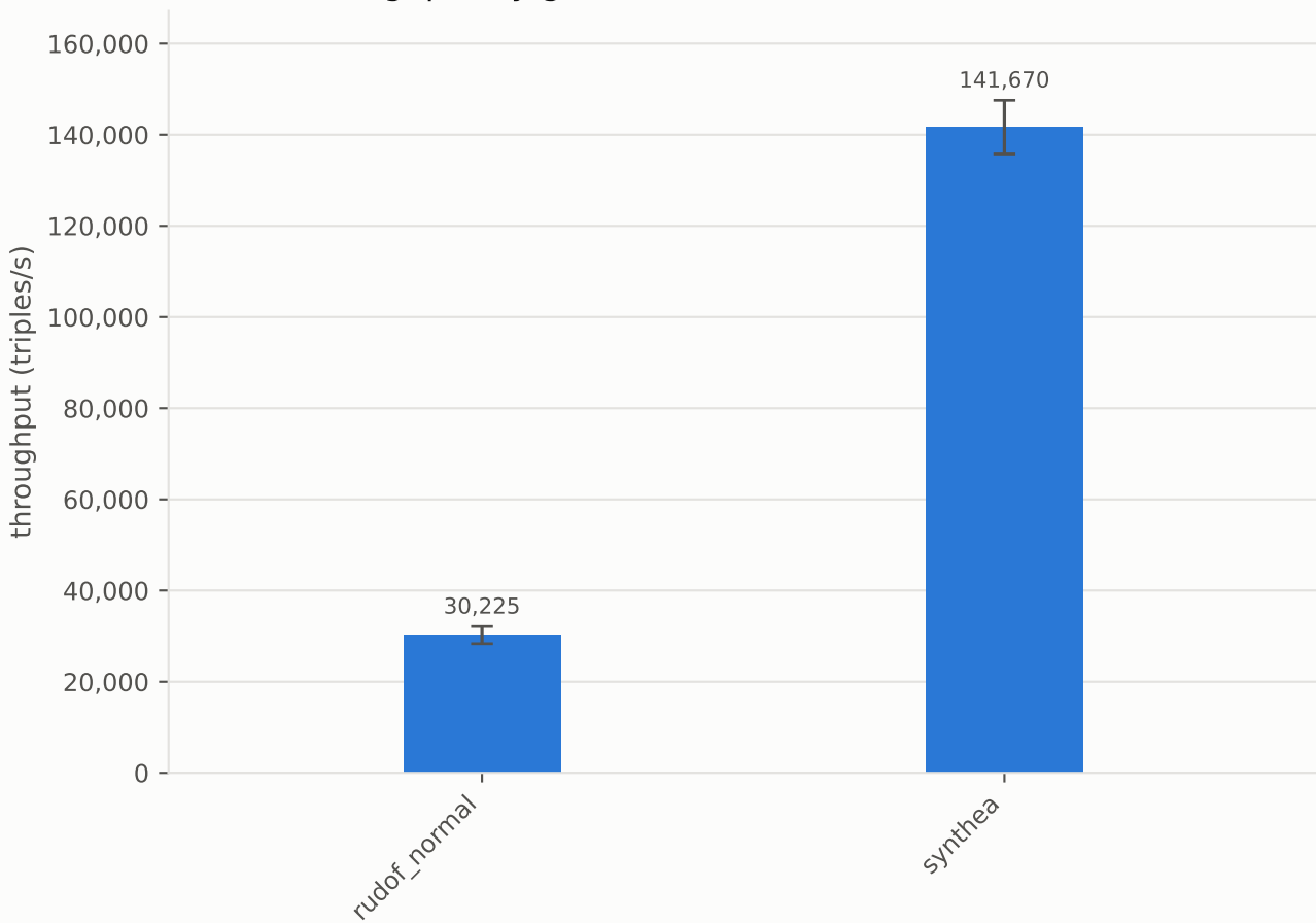
Throughput by generator - mean +/- std over 10 run(s)
