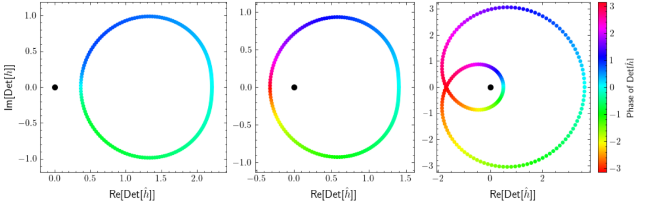
Figure 7.4: Topology of the SP-SSH lattice for \Delta\beta = 0 . Determinant of the block matrix \hat{h} for quasimomenta -\frac{\pi}{a} \leq k < \frac{\pi}{a} . Exactly three distinct topological phases are observed.
