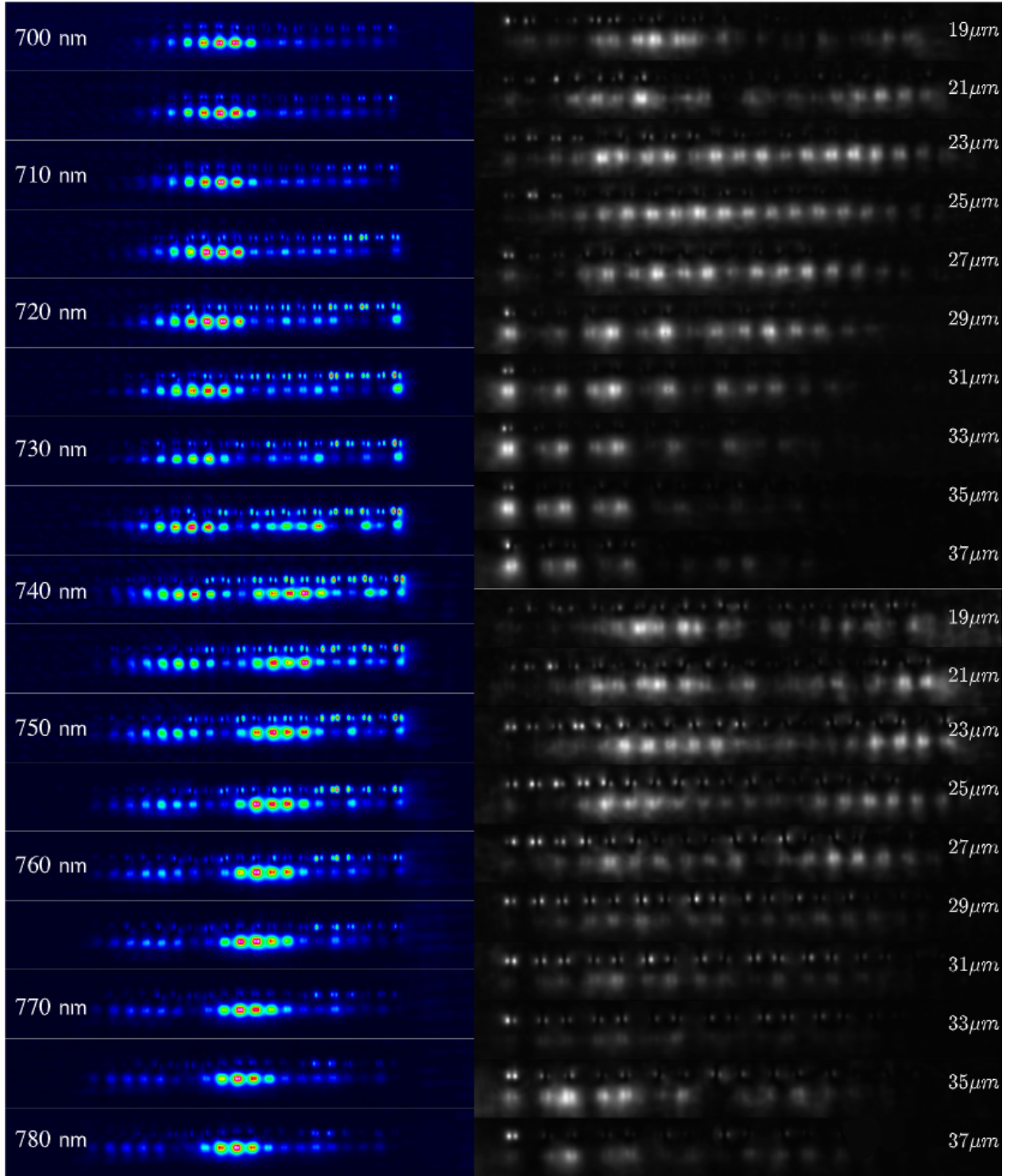
Figure 7.7: Left: Homogeneous SP-SSH lattice ( dx_1 = dx_2 ) for different wavelengths. Right: Top: Excitation at 680 nm for different dimerizations. Bottom: Same excitation at 725 nm.
