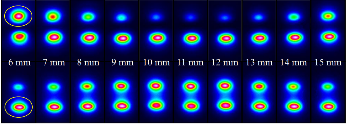
Figure 6.3: Output profiles for different propagation lengths z_i , exciting the upper waveguide (left) and lower waveguide (right), with d = 18 \mu\text{m} .
