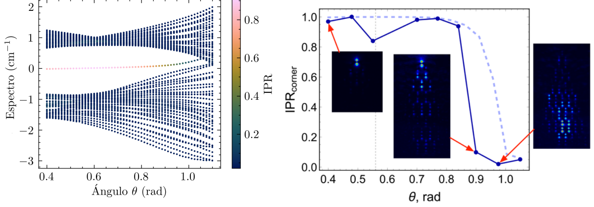
Figure 5.5: Left: Spectrum of the matrix \hat{H}_\Sigma as a function of the angle. Each point is colored according to its inverse participation ratio (IPR). Right: Inverse participation ratio for the corner site excitation as a function of the angle \theta .
