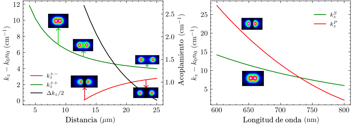
Figure 7.2: Left: Propagation constants and couplings as a function of distance for fundamental modes, calculated using EME. Right: Propagation constants of S and P modes as a function of wavelength.
