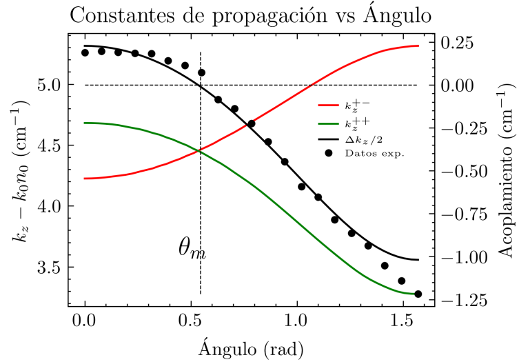
Figure 5.2: Propagation constants and couplings as a function of the angle for p_y modes, numerically calculated using EME. The results are compared with experimental data extracted from Figure 5.1.
