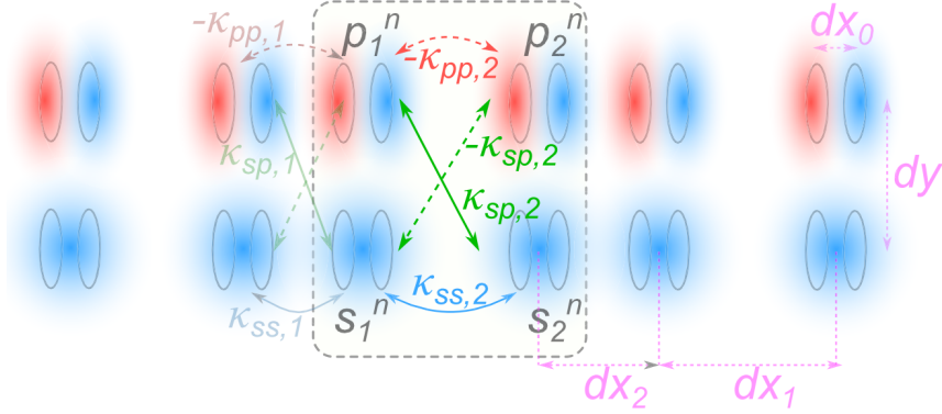
Figure 7.3: Schematic of the SP-SSH lattice and the considered couplings.
