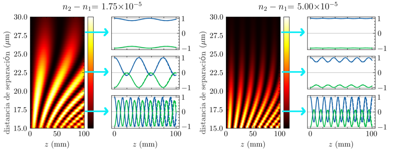
Figure 6.2: Absolute average of intensity imbalances \bar{I}(z) as a function of propagation distance z and the separation distance between waveguides, comparing two regimes: (1) weak asymmetry ( \Delta n = 1.75 \times 10^{-5} ) and (2) strong asymmetry ( \Delta n = 5.00 \times 10^{-5} ). The values I^L (green) and I^R (blue) corresponding to three specific study cases are included.
