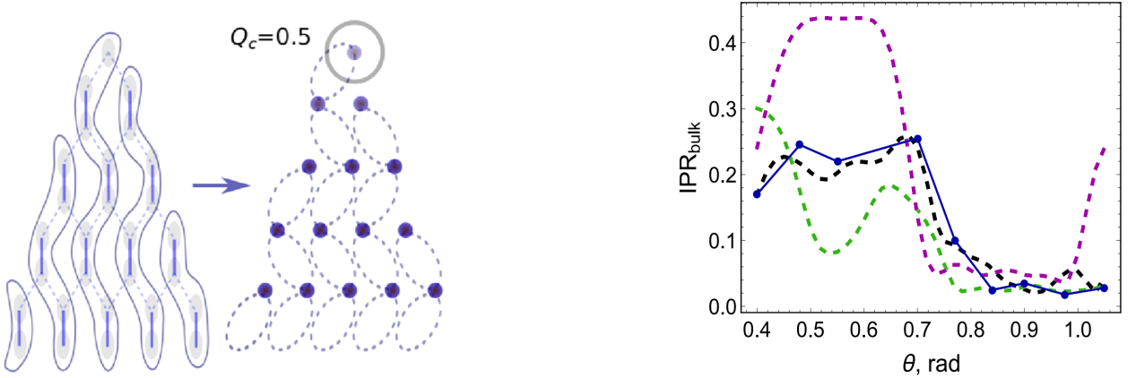
Figure 5.6: Left: Decomposition of the lattice in the flat-band limit into isolated dimer SSH chains. Right: IPR for the experimental excitation of the central site of the lattice (points connected with lines to guide the eye) and numerically simulated for three cases: without long-range couplings and non-orthogonal corrections (dashed purple curve), with long-range couplings but without non-orthogonal corrections (dashed green curve), and with long-range couplings and non-orthogonal corrections (dashed black curve).
