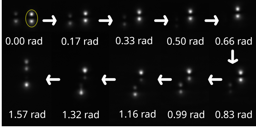
Figure 5.1: Experimental angular sweep for a propagation distance of 15 mm. The effect of the magic angle is observed between 0.50 and 0.66 rad.
