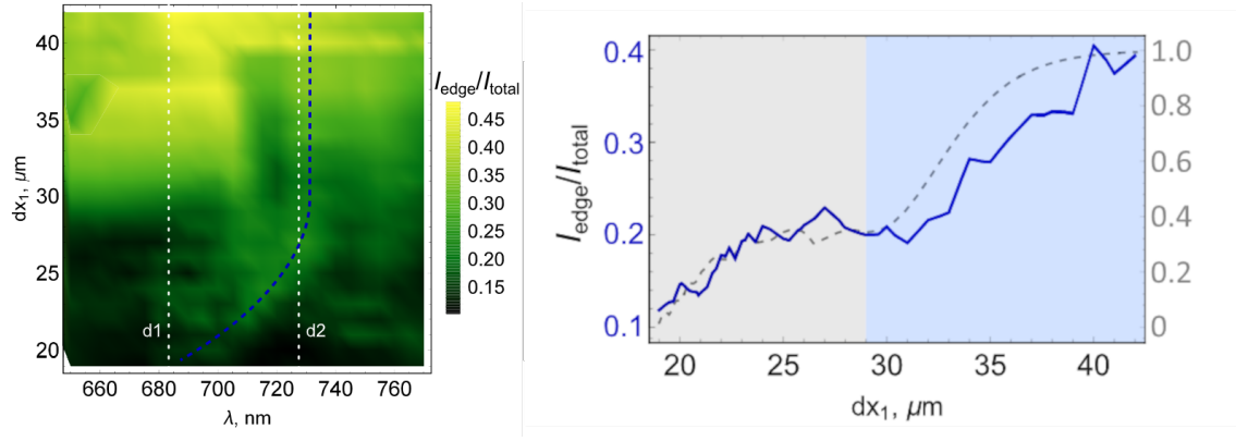
Figure 7.6: Left: Experimental results showing the characteristic plateau. Right: Quantitative comparison between experimental data (solid line) and simulations (dashed line).
