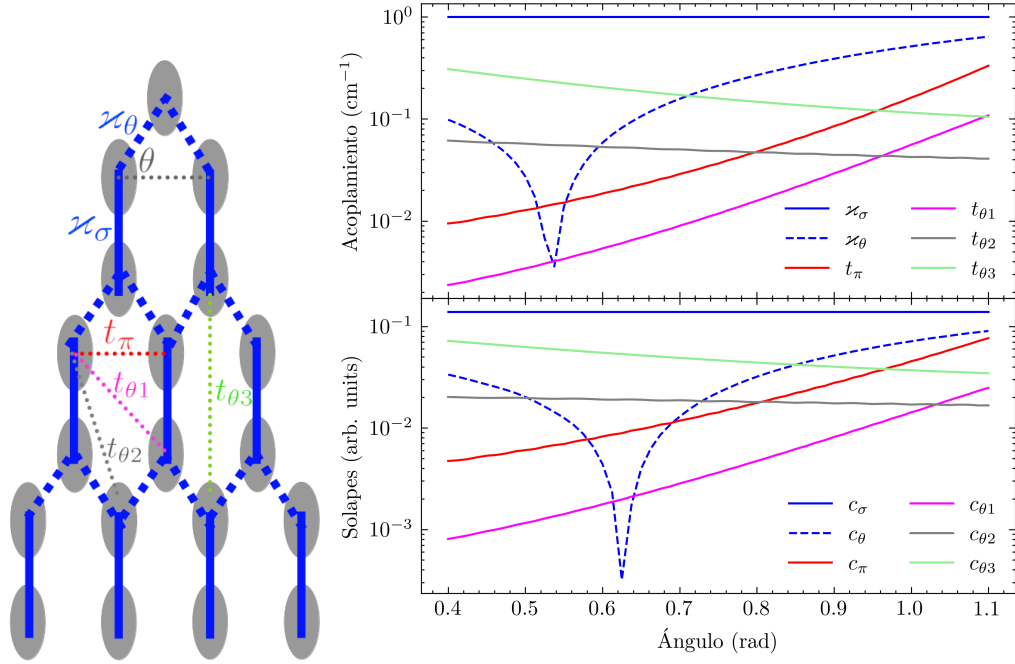
Figure 5.4: Left: Schematic of the honeycomb model for p_y modes with couplings up to third neighbors. Right: (Top) Absolute values of the couplings as a function of the angle \theta . (Bottom) Normalized overlap integrals as a function of the angle \theta .
